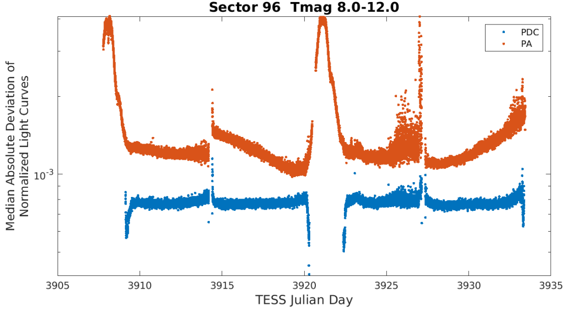
Figure 4: Median absolute deviation (MAD) for the two-minute cadence data from Sector 96, showing the performance of the cotrending after identifying Manual Exclude data quality flags. The MAD is calculated in each cadence across stars with flux variations less than 1% for both the PA (red) and PDC (blue) light curves, where each light curve is normalized by its median flux value. The scatter in the PA light curves is much higher than that for the PDC light curves, and the outliers in the PA light curves are largely absent from the PDC light curves due to the use of the anomaly flags.
