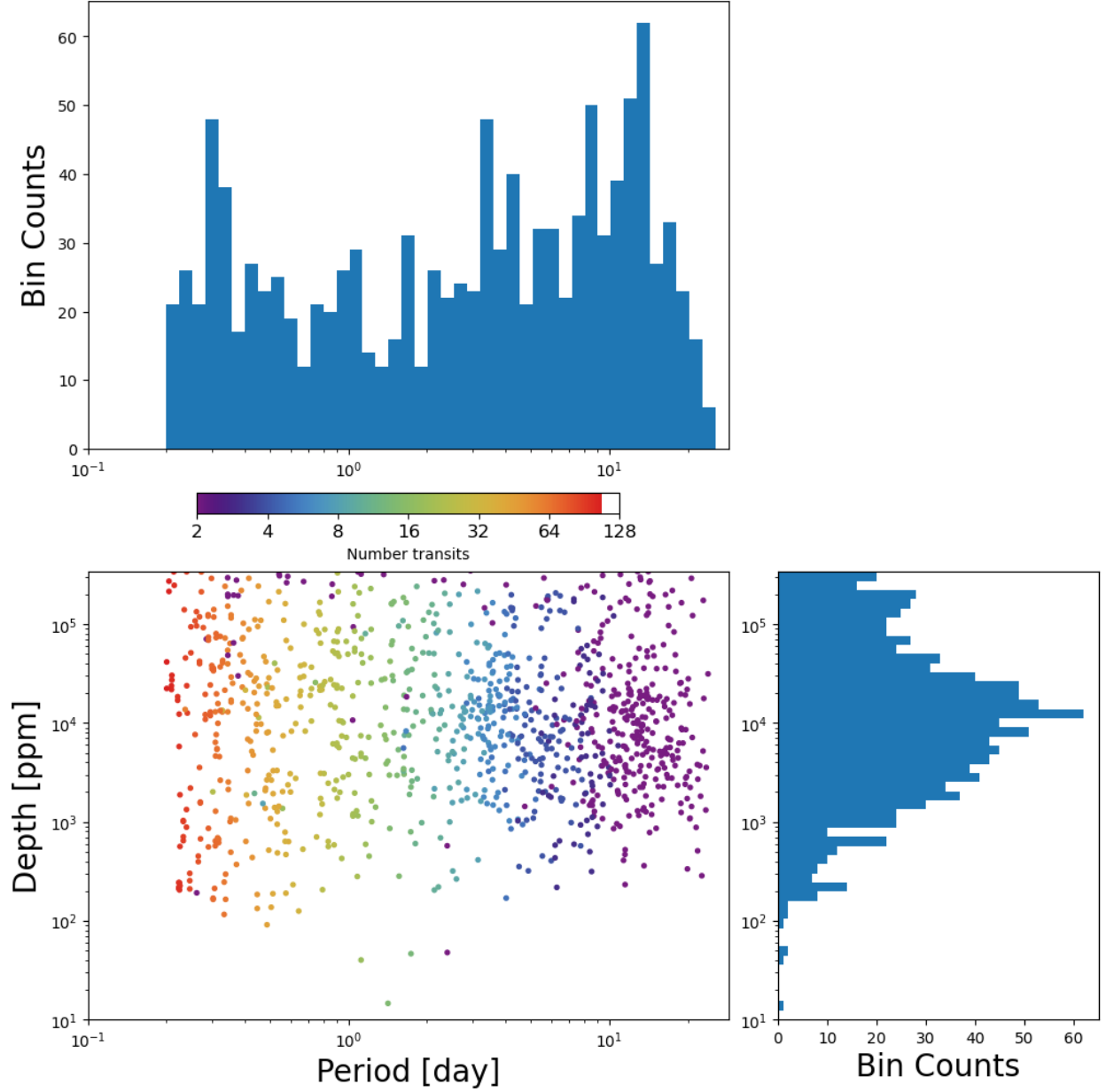
Figure 7: Lower Left Panel: Transit depth as a function of orbital period for the 1149 TCEs identified for the Sector 96 search. Reported depth comes from the DV limb-darkened transit fit depth when available, and the DV trapezoid model fit depth when not available. The number of observed transit events for each TCE is indicated by point color. Top Panel: Orbital period distribution of the TCEs shown in the lower left panel. Right Panel: Transit depth distribution for the TCEs shown in the lower left panel.
