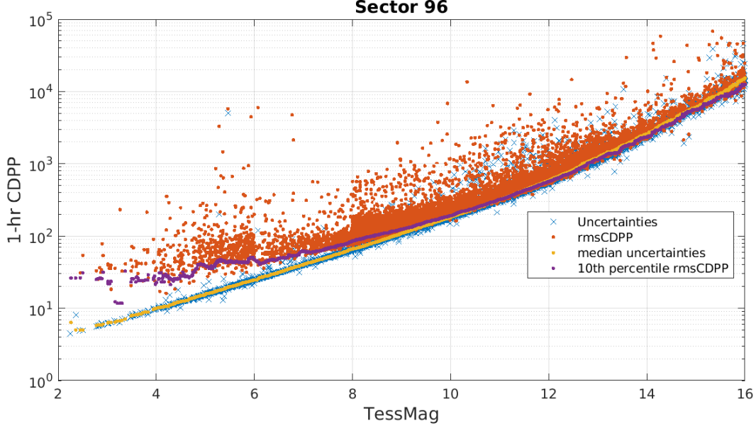
Figure 5: 1-hour CDPP. The red points are the RMS CDPP measurements for the 12994 light curves from Sector 96 plotted as a function of TESS magnitude. The blue x’s are the uncertainties, scaled to 1-hour timescale. The purple curve is a moving 10th percentile of the RMS CDPP measurements, and the gold curve is a moving median of the 1-hr uncertainties.
