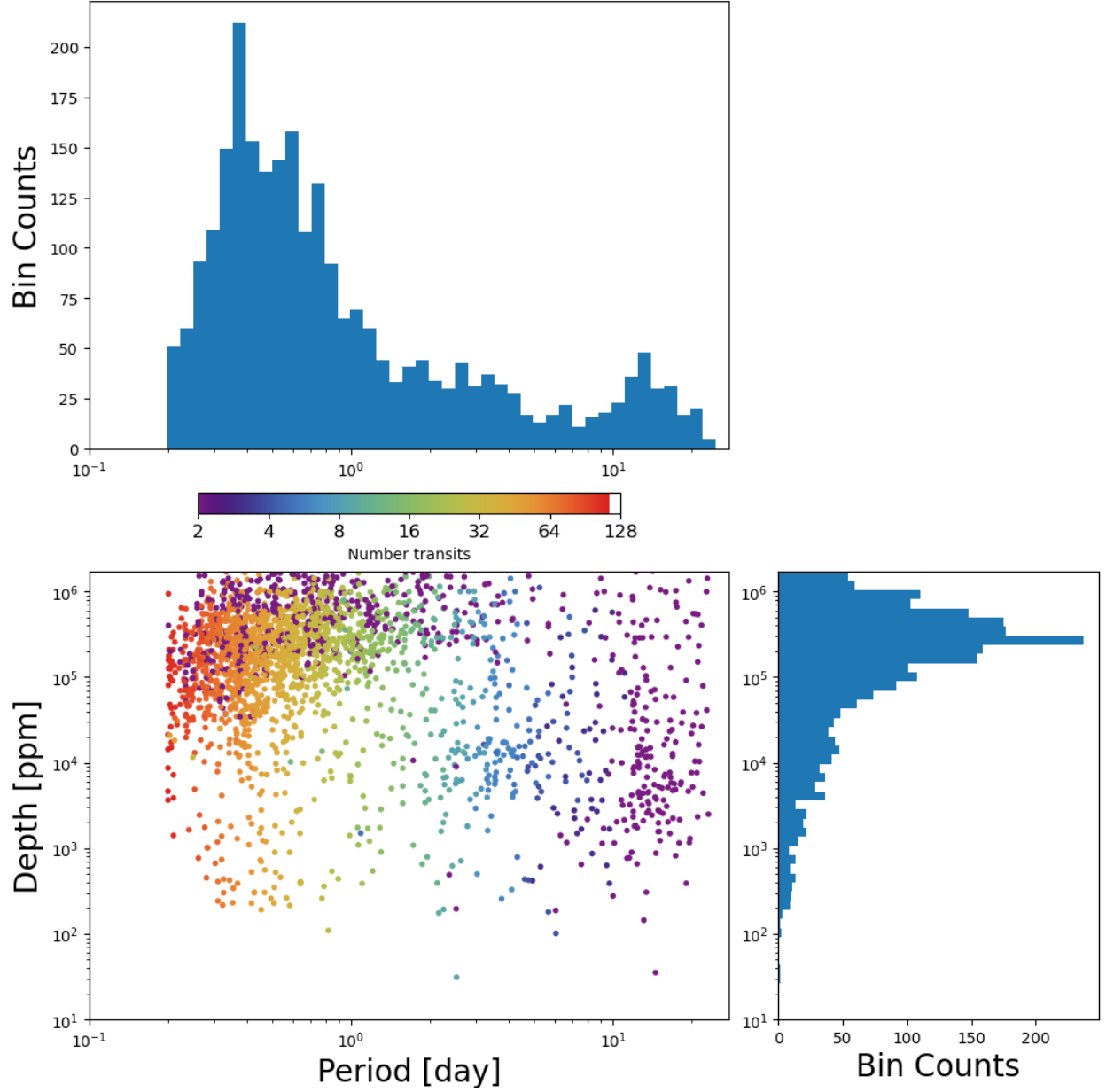
Figure 7: Lower Left Panel: Transit depth as a function of orbital period for the 2514 TCEs identified for the Sector 92 search. Reported depth comes from the DV limb-darkened transit fit depth when available, and the DV trapezoid model fit depth when not available. The number of observed transit events for each TCE is indicated by point color. Top Panel: Orbital period distribution of the TCEs shown in the lower left panel. Right Panel: Transit depth distribution for the TCEs shown in the lower left panel.
