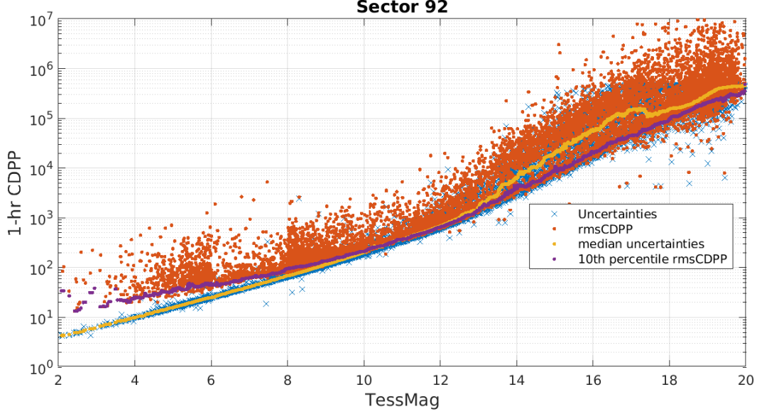
Figure 5: 1-hour CDPP. The red points are the RMS CDPP measurements for the 12999 light curves from Sector 92 plotted as a function of TESS magnitude. The blue x’s are the uncertainties, scaled to 1-hour timescale. The purple curve is a moving 10th percentile of the RMS CDPP measurements, and the gold curve is a moving median of the 1-hr uncertainties.
