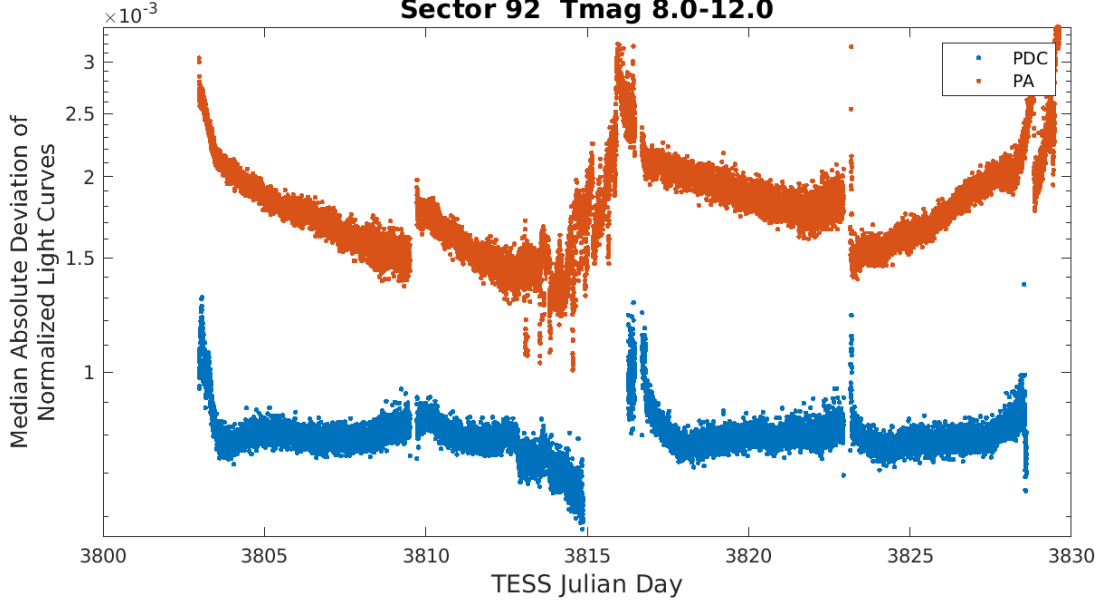
Figure 4: Median absolute deviation (MAD) for the two-minute cadence data from Sector 92, showing the performance of the cotrending after identifying Manual Exclude data quality flags. The MAD is calculated in each cadence across stars with flux variations less than 1% for both the PA (red) and PDC (blue) light curves, where each light curve is normalized by its median flux value. The scatter in the PA light curves is much higher than that for the PDC light curves, and the outliers in the PA light curves are largely absent from the PDC light curves due to the use of the anomaly flags.
