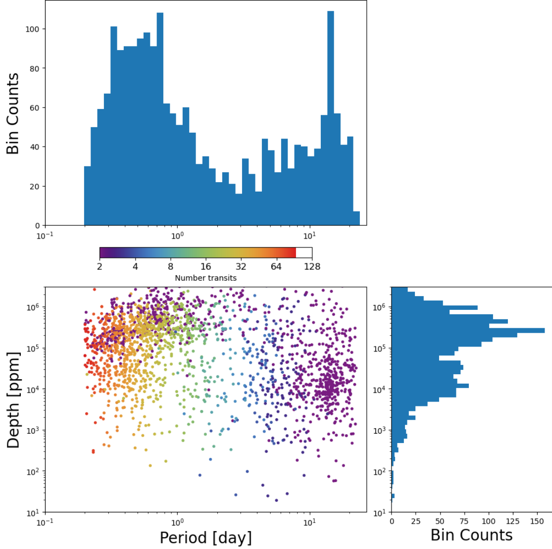
Figure 7: Lower Left Panel: Transit depth as a function of orbital period for the 2157 TCEs identified for the Sector 91 search. Reported depth comes from the DV limb-darkened transit fit depth when available, and the DV trapezoid model fit depth when not available. The number of observed transit events for each TCE is indicated by point color. Top Panel: Orbital period distribution of the TCEs shown in the lower left panel. Right Panel: Transit depth distribution for the TCEs shown in the lower left panel.
