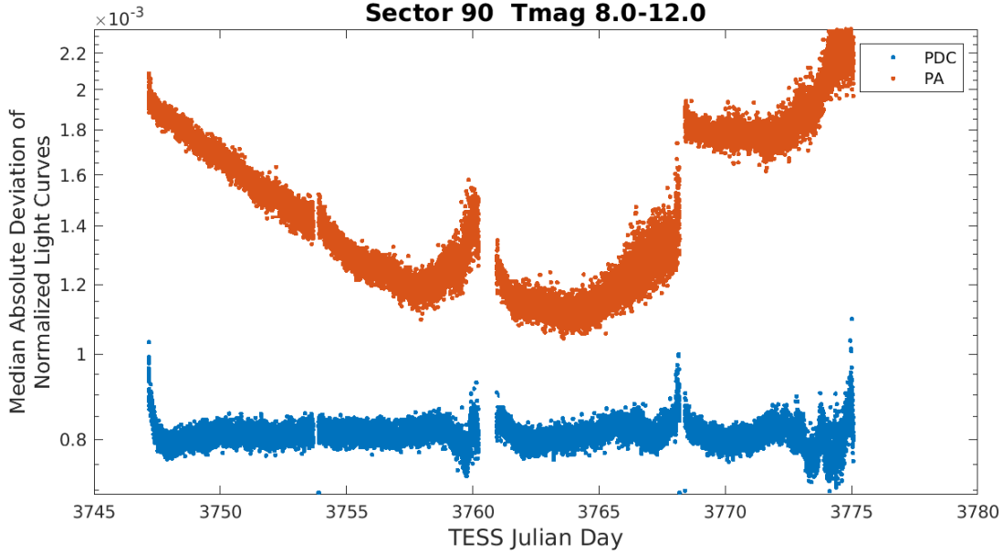
Figure 4: Median absolute deviation (MAD) for the two-minute cadence data from Sector 90, showing the performance of the cotrending after identifying Manual Exclude data quality flags. The MAD is calculated in each cadence across stars with flux variations less than 1% for both the PA (red) and PDC (blue) light curves, where each light curve is normalized by its median flux value. The scatter in the PA light curves is much higher than that for the PDC light curves, and the outliers in the PA light curves are largely absent from the PDC light curves due to the use of the anomaly flags.
