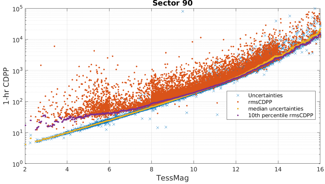
Figure 5: 1-hour CDPP. The red points are the RMS CDPP measurements for the 12995 light curves from Sector 90 plotted as a function of TESS magnitude. The blue x’s are the uncertainties, scaled to 1-hour timescale. The purple curve is a moving 10th percentile of the RMS CDPP measurements, and the gold curve is a moving median of the 1-hr uncertainties.
