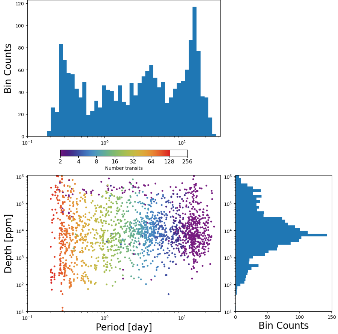
Figure 7: Lower Left Panel: Transit depth as a function of orbital period for the 1904 TCEs identified for the Sector 90 search. Reported depth comes from the DV limb-darkened transit fit depth when available, and the DV trapezoid model fit depth when not available. The number of observed transit events for each TCE is indicated by point color. Top Panel: Orbital period distribution of the TCEs shown in the lower left panel. Right Panel: Transit depth distribution for the TCEs shown in the lower left panel.
