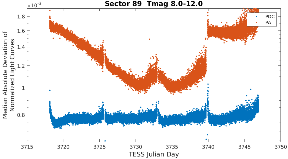
Figure 4: Median absolute deviation (MAD) for the two-minute cadence data from Sector 89, showing the performance of the cotrending after identifying Manual Exclude data quality flags. The MAD is calculated in each cadence across stars with flux variations less than 1% for both the PA (red) and PDC (blue) light curves, where each light curve is normalized by its median flux value. The scatter in the PA light curves is much higher than that for the PDC light curves, and the outliers in the PA light curves are largely absent from the PDC light curves due to the use of the anomaly flags.
