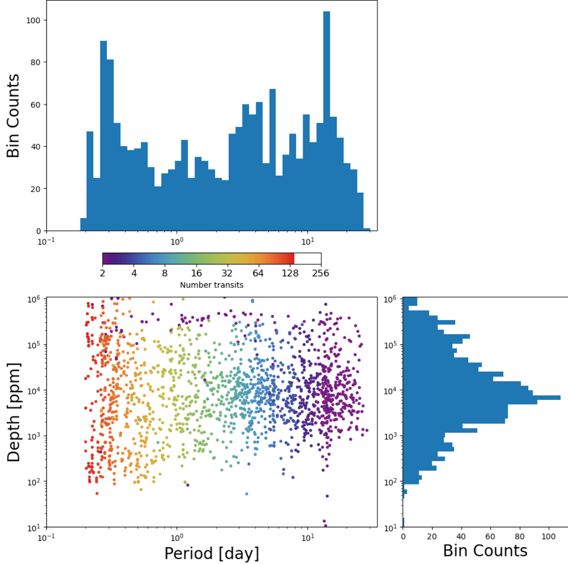
Figure 7: Lower Left Panel: Transit depth as a function of orbital period for the 1755 TCEs identified for the Sector 89 search. Reported depth comes from the DV limb-darkened transit fit depth when available, and the DV trapezoid model fit depth when not available. The number of observed transit events for each TCE is indicated by point color. Top Panel: Orbital period distribution of the TCEs shown in the lower left panel. Right Panel: Transit depth distribution for the TCEs shown in the lower left panel.
