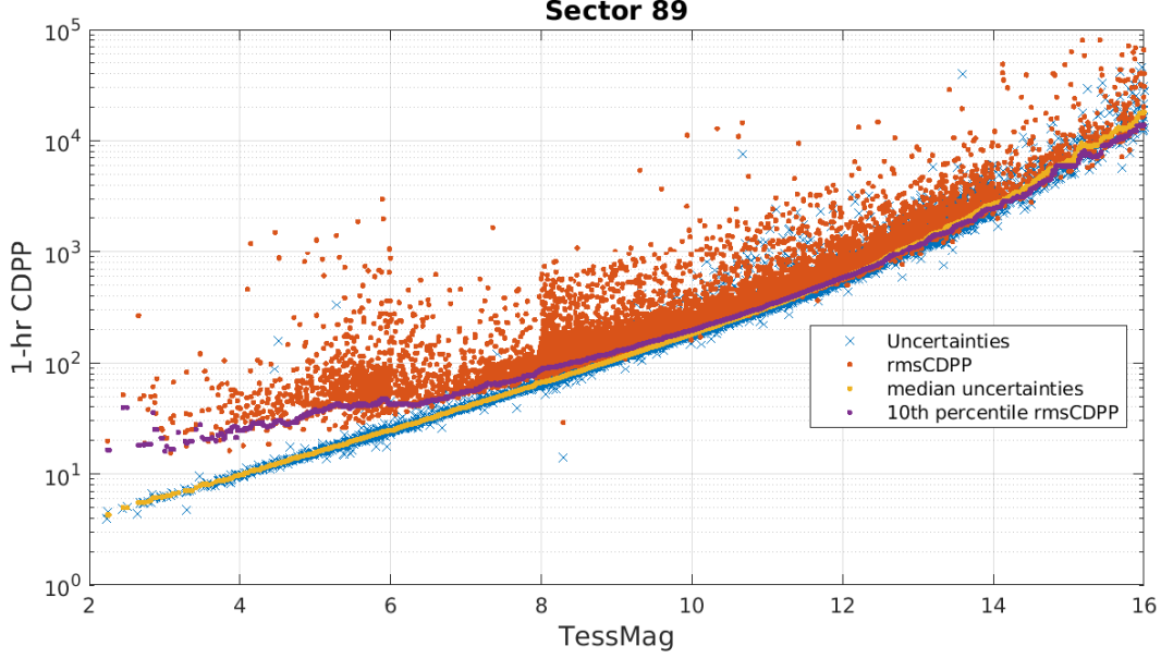
Figure 5: 1-hour CDPP. The red points are the RMS CDPP measurements for the 12995 light curves from Sector 89 plotted as a function of TESS magnitude. The blue x’s are the uncertainties, scaled to 1-hour timescale. The purple curve is a moving 10th percentile of the RMS CDPP measurements, and the gold curve is a moving median of the 1-hr uncertainties.
