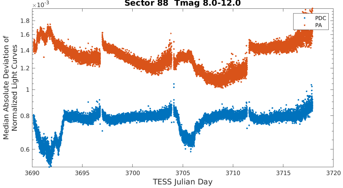
Figure 4: Median absolute deviation (MAD) for the two-minute cadence data from Sector 88, showing the performance of the cotrending after identifying Manual Exclude data quality flags. The MAD is calculated in each cadence across stars with flux variations less than 1% for both the PA (red) and PDC (blue) light curves, where each light curve is normalized by its median flux value. The scatter in the PA light curves is much higher than that for the PDC light curves, and the outliers in the PA light curves are largely absent from the PDC light curves due to the use of the anomaly flags.
