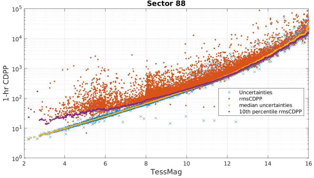
Figure 5: 1-hour CDPP. The red points are the RMS CDPP measurements for the 12993 light curves from Sector 88 plotted as a function of TESS magnitude. The blue x's are the uncertainties, scaled to 1-hour timescale. The purple curve is a moving 10th percentile of the RMS CDPP measurements, and the gold curve is a moving median of the 1-hr uncertainties.
