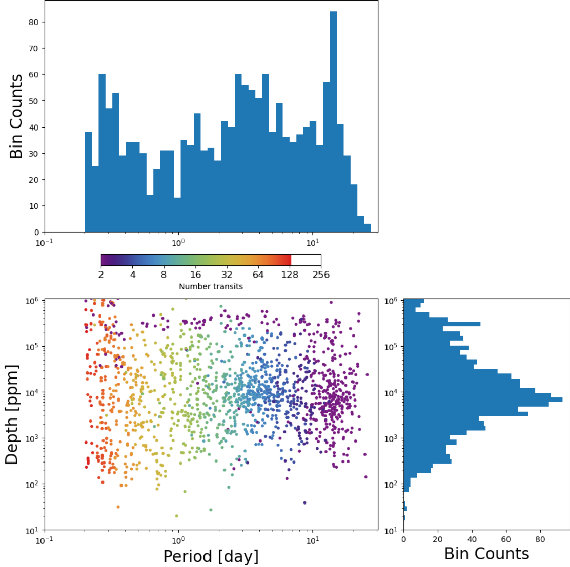
Figure 7: Lower Left Panel: Transit depth as a function of orbital period for the 1576 TCEs identified for the Sector 88 search. Reported depth comes from the DV limb-darkened transit fit depth when available, and the DV trapezoid model fit depth when not available. The number of observed transit events for each TCE is indicated by point color. Top Panel: Orbital period distribution of the TCEs shown in the lower left panel. Right Panel: Transit depth distribution for the TCEs shown in the lower left panel.
