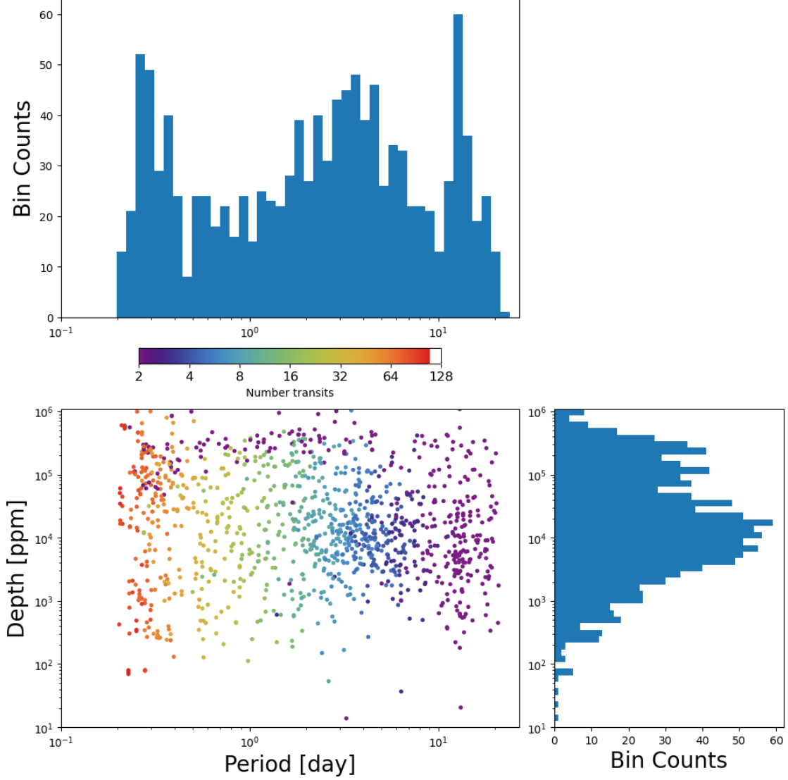
Figure 7: Lower Left Panel: Transit depth as a function of orbital period for the 1186 TCEs identified for the Sector 85 search. Reported depth comes from the DV limb-darkened transit fit depth when available, and the DV trapezoid model fit depth when not available. The number of observed transit events for each TCE is indicated by point color. Top Panel: Orbital period distribution of the TCEs shown in the lower left panel. Right Panel: Transit depth distribution for the TCEs shown in the lower left panel.
