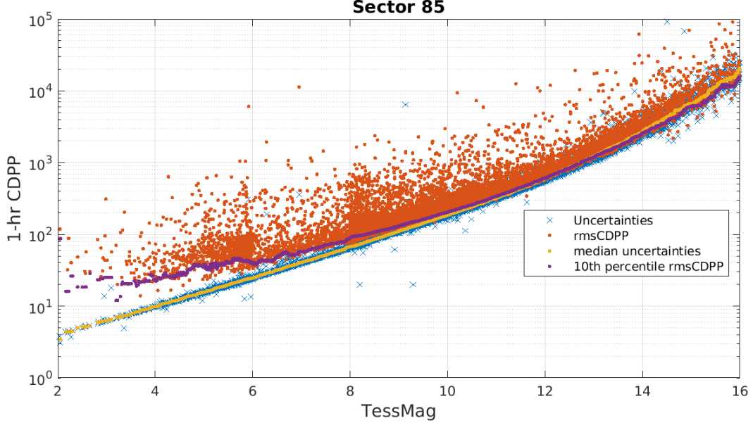
Figure 5: 1-hour CDPP. The red points are the RMS CDPP measurements for the 12993 light curves from Sector 85 plotted as a function of TESS magnitude. The blue x’s are the uncertainties, scaled to 1-hour timescale. The purple curve is a moving 10th percentile of the RMS CDPP measurements, and the gold curve is a moving median of the 1-hr uncertainties.
