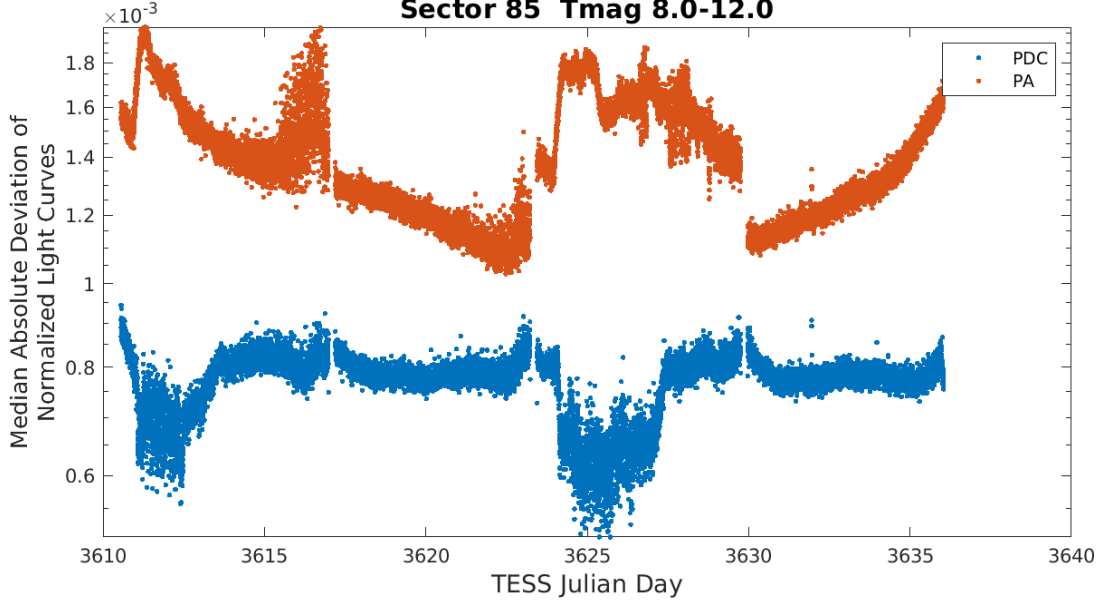
Figure 4: Median absolute deviation (MAD) for the two-minute cadence data from Sector 85, showing the performance of the cotrending after identifying Manual Exclude data quality flags. The MAD is calculated in each cadence across stars with flux variations less than 1% for both the PA (red) and PDC (blue) light curves, where each light curve is normalized by its median flux value. The scatter in the PA light curves is much higher than that for the PDC light curves, and the outliers in the PA light curves are largely absent from the PDC light curves due to the use of the anomaly flags.
