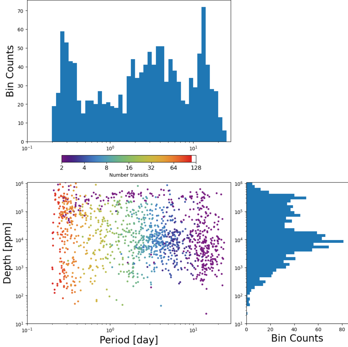
Figure 7: Lower Left Panel: Transit depth as a function of orbital period for the 1355 TCEs identified for the Sector 84 search. Reported depth comes from the DV limb-darkened transit fit depth when available, and the DV trapezoid model fit depth when not available. The number of observed transit events for each TCE is indicated by point color. Top Panel: Orbital period distribution of the TCEs shown in the lower left panel. Right Panel: Transit depth distribution for the TCEs shown in the lower left panel.
