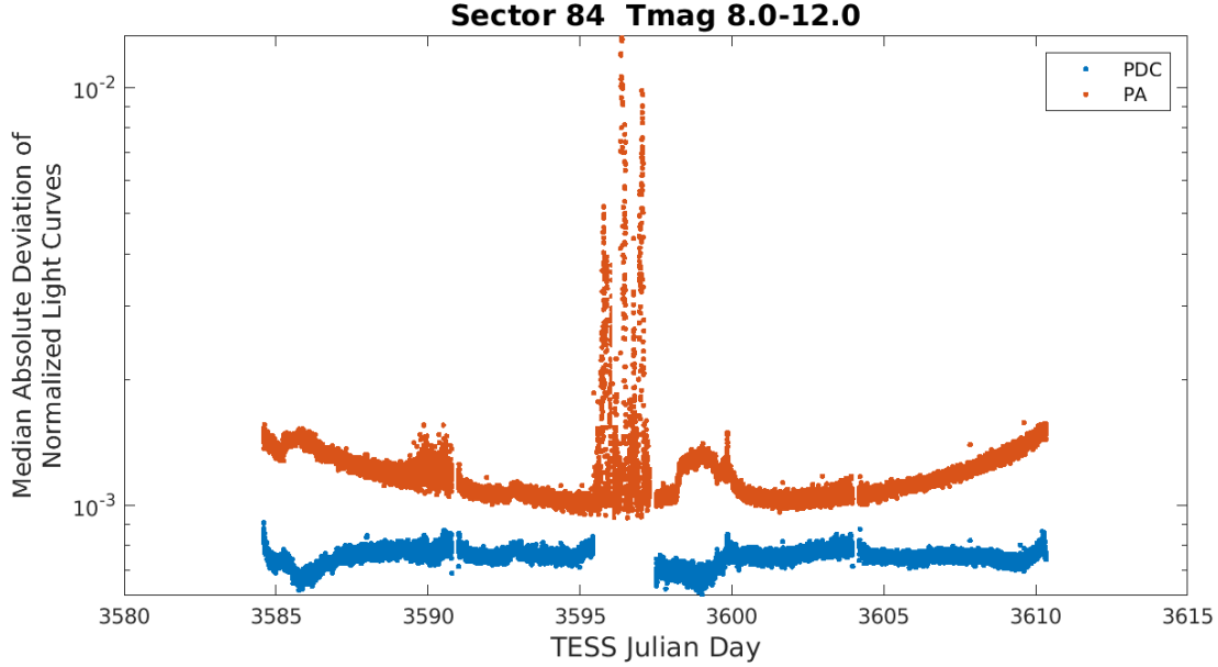
Figure 4: Median absolute deviation (MAD) for the two-minute cadence data from Sector 84, showing the performance of the cotrending after identifying Manual Exclude data quality flags. The MAD is calculated in each cadence across stars with flux variations less than 1% for both the PA (red) and PDC (blue) light curves, where each light curve is normalized by its median flux value. The scatter in the PA light curves is much higher than that for the PDC light curves, and the outliers in the PA light curves are largely absent from the PDC light curves due to the use of the anomaly flags.
