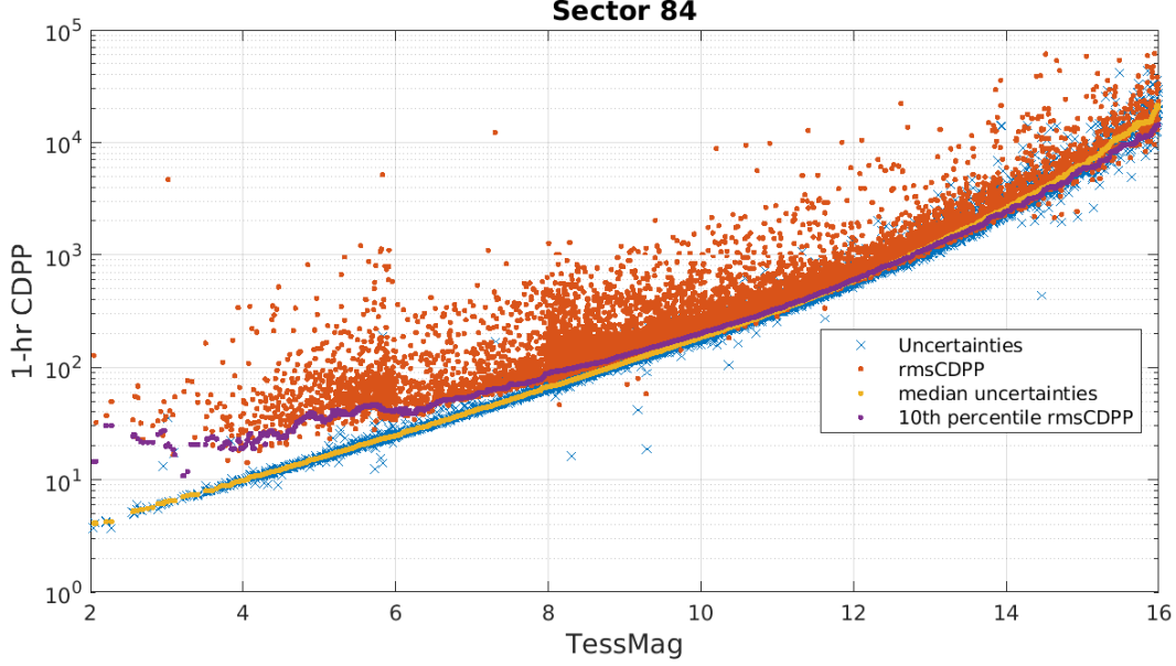
Figure 5: 1-hour CDPP. The red points are the RMS CDPP measurements for the 12997 light curves from Sector 84 plotted as a function of TESS magnitude. The blue x’s are the uncertainties, scaled to 1-hour timescale. The purple curve is a moving 10th percentile of the RMS CDPP measurements, and the gold curve is a moving median of the 1-hr uncertainties.
