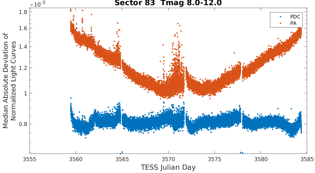
Figure 4: Median absolute deviation (MAD) for the two-minute cadence data from Sector 83, showing the performance of the cotrending after identifying Manual Exclude data quality flags. The MAD is calculated in each cadence across stars with flux variations less than 1% for both the PA (red) and PDC (blue) light curves, where each light curve is normalized by its median flux value. The scatter in the PA light curves is much higher than that for the PDC light curves, and the outliers in the PA light curves are largely absent from the PDC light curves due to the use of the anomaly flags.
