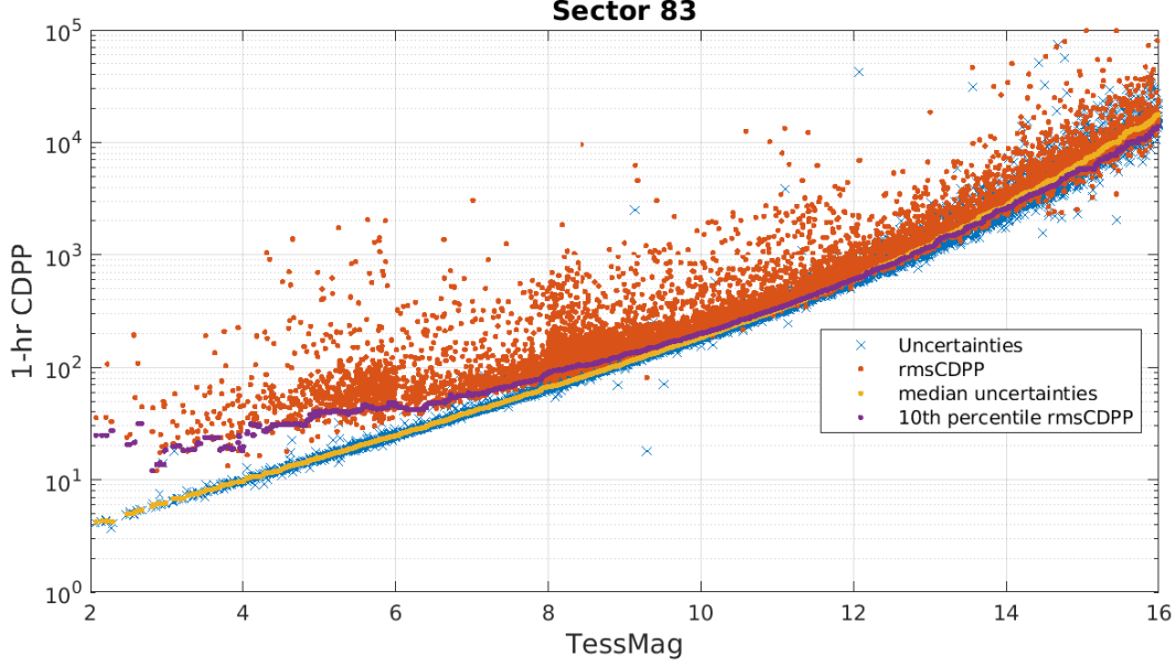
Figure 5: 1-hour CDPP. The red points are the RMS CDPP measurements for the 12997 light curves from Sector 83 plotted as a function of TESS magnitude. The blue x’s are the uncertainties, scaled to 1-hour timescale. The purple curve is a moving 10th percentile of the RMS CDPP measurements, and the gold curve is a moving median of the 1-hr uncertainties.
