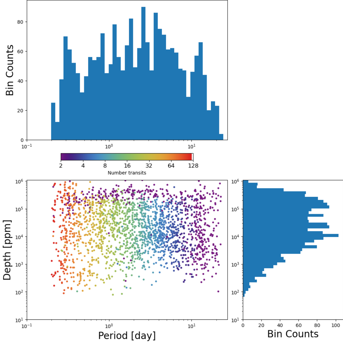
Figure 7: Lower Left Panel: Transit depth as a function of orbital period for the 2180 TCEs identified for the Sector 83 search. Reported depth comes from the DV limb-darkened transit fit depth when available, and the DV trapezoid model fit depth when not available. The number of observed transit events for each TCE is indicated by point color. Top Panel: Orbital period distribution of the TCEs shown in the lower left panel. Right Panel: Transit depth distribution for the TCEs shown in the lower left panel.
