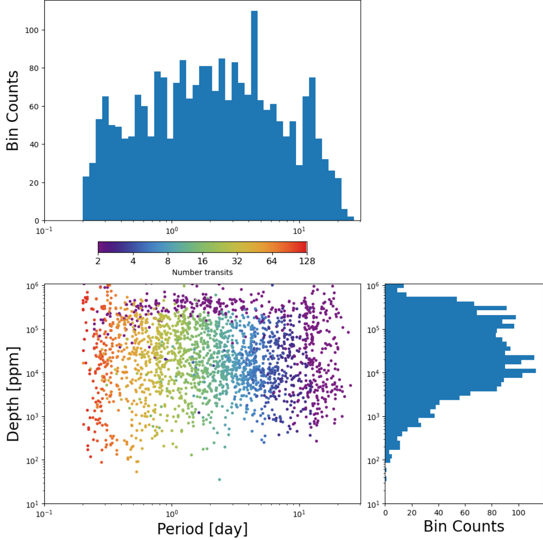
Figure 7: Lower Left Panel: Transit depth as a function of orbital period for the 2353 TCEs identified for the Sector 82 search. Reported depth comes from the DV limb-darkened transit fit depth when available, and the DV trapezoid model fit depth when not available. The number of observed transit events for each TCE is indicated by point color. Top Panel: Orbital period distribution of the TCEs shown in the lower left panel. Right Panel: Transit depth distribution for the TCEs shown in the lower left panel.
