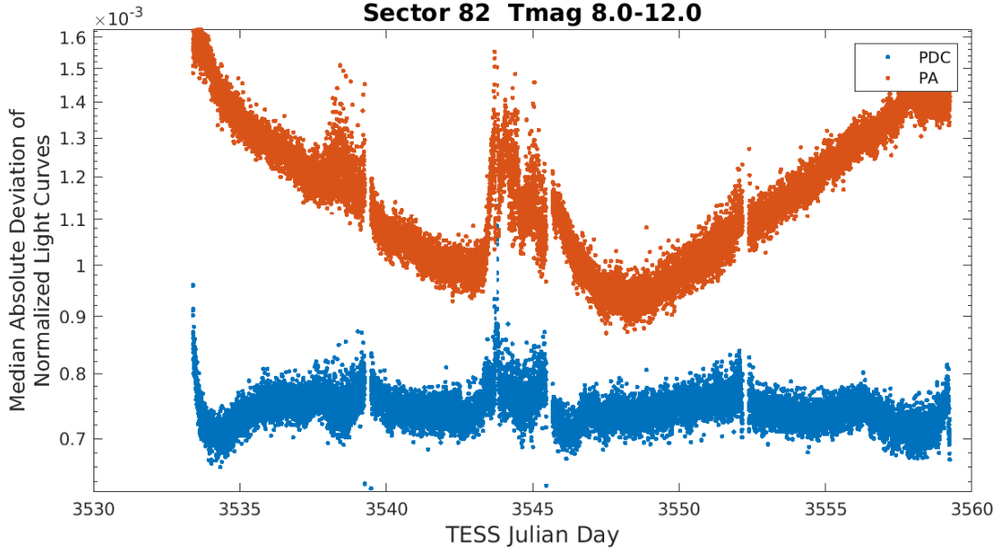
Figure 4: Median absolute deviation (MAD) for the two-minute cadence data from Sector 82, showing the performance of the cotrending after identifying Manual Exclude data quality flags. The MAD is calculated in each cadence across stars with flux variations less than 1% for both the PA (red) and PDC (blue) light curves, where each light curve is normalized by its median flux value. The scatter in the PA light curves is much higher than that for the PDC light curves, and the outliers in the PA light curves are largely absent from the PDC light curves due to the use of the anomaly flags.
