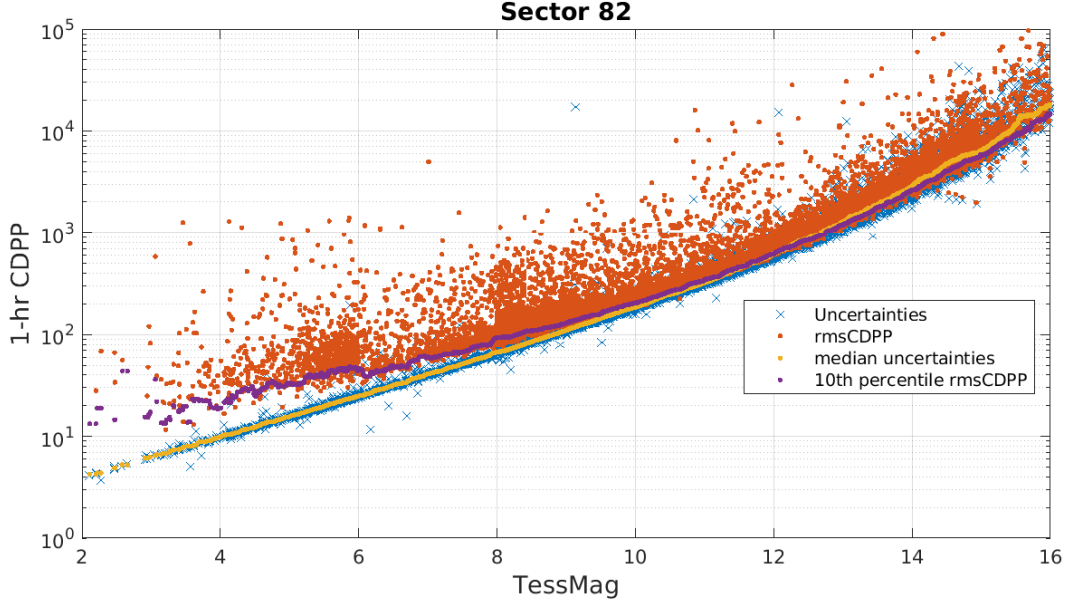
Figure 5: 1-hour CDPP. The red points are the RMS CDPP measurements for the 12997 light curves from Sector 82 plotted as a function of TESS magnitude. The blue x's are the uncertainties, scaled to 1-hour timescale. The purple curve is a moving 10th percentile of the RMS CDPP measurements, and the gold curve is a moving median of the 1-hr uncertainties.
