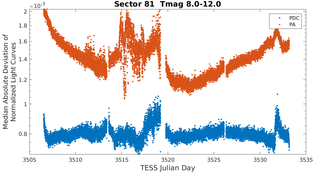
Figure 4: Median absolute deviation (MAD) for the two-minute cadence data from Sector 81, showing the performance of the cotrending after identifying Manual Exclude data quality flags. The MAD is calculated in each cadence across stars with flux variations less than 1% for both the PA (red) and PDC (blue) light curves, where each light curve is normalized by its median flux value. The scatter in the PA light curves is much higher than that for the PDC light curves, and the outliers in the PA light curves are largely absent from the PDC light curves due to the use of the anomaly flags.
