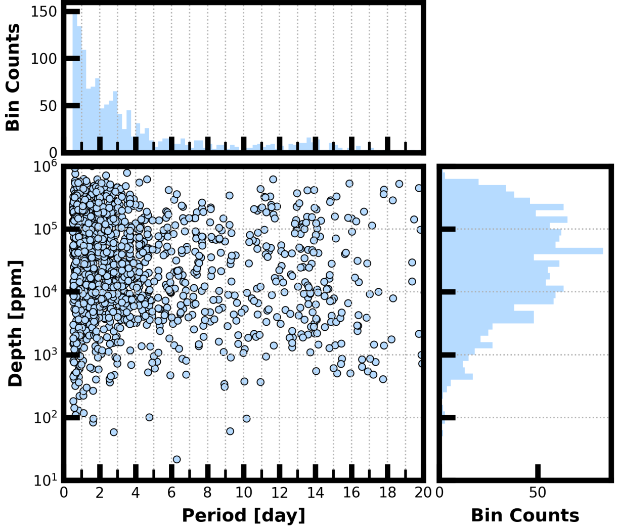
Figure 7: Lower Left Panel: Transit depth as a function of orbital period for the 1731 TCEs identified for the Sector 80 search. For enhanced visibility of long period detections, TCEs with orbital period < 0.5 days are not shown. Reported depth comes from the DV limb-darkened transit fit depth when available, and the DV trapezoid model fit depth when not available. Top Panel: Orbital period distribution of the TCEs shown in the lower left panel. Right Panel: Transit depth distribution for the TCEs shown in the lower left panel.
