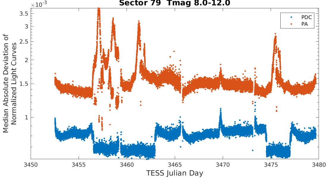
Figure 4: Median absolute deviation (MAD) for the two-minute cadence data from Sector 79, showing the performance of the cotrending after identifying Manual Exclude data quality flags. The MAD is calculated in each cadence across stars with flux variations less than 1% for both the PA (red) and PDC (blue) light curves, where each light curve is normalized by its median flux value. The scatter in the PA light curves is much higher than that for the PDC light curves, and the outliers in the PA light curves are largely absent from the PDC light curves due to the use of the anomaly flags.
