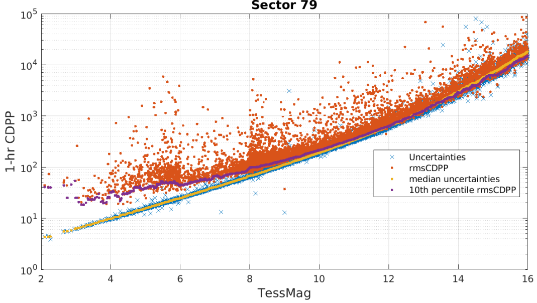
Figure 5: 1-hour CDPP. The red points are the RMS CDPP measurements for the 11712 light curves from Sector 79 plotted as a function of TESS magnitude. The blue x’s are the uncertainties, scaled to 1-hour timescale. The purple curve is a moving 10th percentile of the RMS CDPP measurements, and the gold curve is a moving median of the 1-hr uncertainties.
