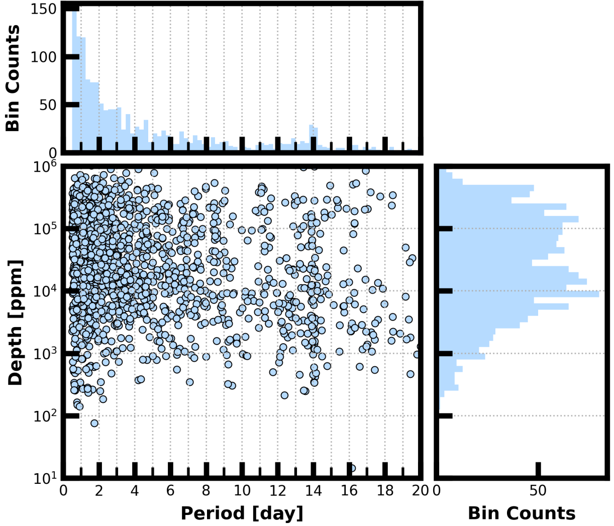
Figure 7: Lower Left Panel: Transit depth as a function of orbital period for the 1877 TCEs identified for the Sector 79 search. For enhanced visibility of long period detections, TCEs with orbital period < 0.5 days are not shown. Reported depth comes from the DV limb-darkened transit fit depth when available, and the DV trapezoid model fit depth when not available. Top Panel: Orbital period distribution of the TCEs shown in the lower left panel. Right Panel: Transit depth distribution for the TCEs shown in the lower left panel.
