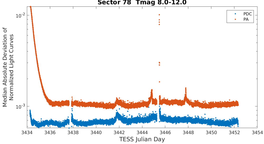
Figure 4: Median absolute deviation (MAD) for the two-minute cadence data from Sector 78, showing the performance of the cotrending after identifying Manual Exclude data quality flags. The MAD is calculated in each cadence across stars with flux variations less than 1% for both the PA (red) and PDC (blue) light curves, where each light curve is normalized by its median flux value. The scatter in the PA light curves is much higher than that for the PDC light curves, and the outliers in the PA light curves are largely absent from the PDC light curves due to the use of the anomaly flags.
