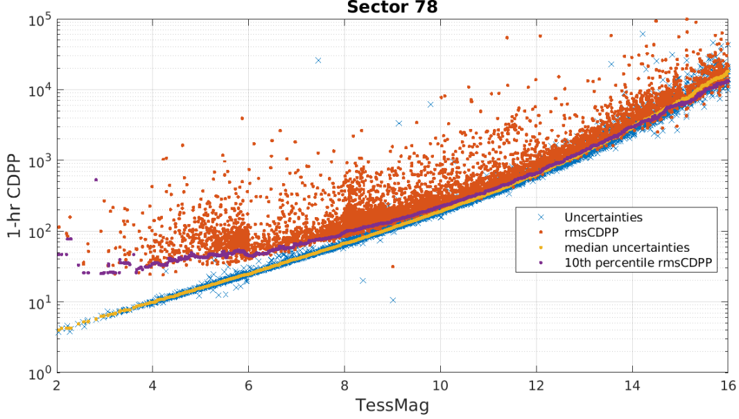
Figure 5: 1-hour CDPP. The red points are the RMS CDPP measurements for the 9923 light curves from Sector 78 plotted as a function of TESS magnitude. The blue x’s are the uncertainties, scaled to 1-hour timescale. The purple curve is a moving 10th percentile of the RMS CDPP measurements, and the gold curve is a moving median of the 1-hr uncertainties.
