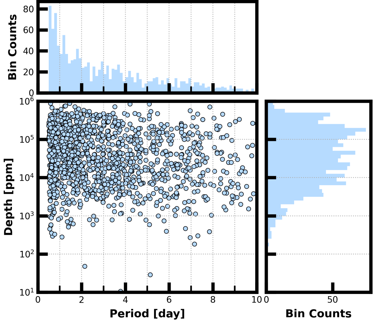
Figure 7: Lower Left Panel: Transit depth as a function of orbital period for the 1580 TCEs identified for the Sector 78 search. For enhanced visibility of long period detections, TCEs with orbital period < 0.5 days are not shown. Reported depth comes from the DV limb-darkened transit fit depth when available, and the DV trapezoid model fit depth when not available. Top Panel: Orbital period distribution of the TCEs shown in the lower left panel. Right Panel: Transit depth distribution for the TCEs shown in the lower left panel.
