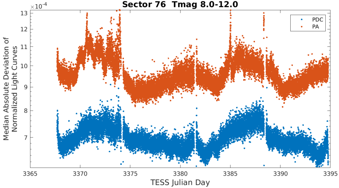
Figure 4: Median absolute deviation (MAD) for the two-minute cadence data from Sector 76, showing the performance of the cotrending after identifying Manual Exclude data quality flags. The MAD is calculated in each cadence across stars with flux variations less than 1% for both the PA (red) and PDC (blue) light curves, where each light curve is normalized by its median flux value. The scatter in the PA light curves is much higher than that for the PDC light curves, and the outliers in the PA light curves are largely absent from the PDC light curves due to the use of the anomaly flags.
