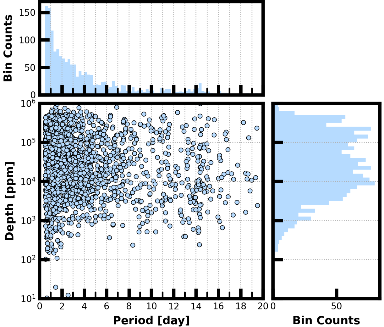
Figure 7: Lower Left Panel: Transit depth as a function of orbital period for the 1965 TCEs identified for the Sector 76 search. For enhanced visibility of long period detections, TCEs with orbital period < 0.5 days are not shown. Reported depth comes from the DV limb-darkened transit fit depth when available, and the DV trapezoid model fit depth when not available. Top Panel: Orbital period distribution of the TCEs shown in the lower left panel. Right Panel: Transit depth distribution for the TCEs shown in the lower left panel.
