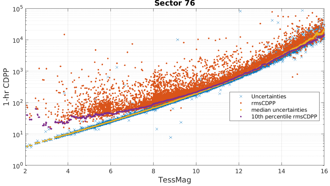
Figure 5: 1-hour CDPP. The red points are the RMS CDPP measurements for the 9952 light curves from Sector 76 plotted as a function of TESS magnitude. The blue x’s are the uncertainties, scaled to 1-hour timescale. The purple curve is a moving 10th percentile of the RMS CDPP measurements, and the gold curve is a moving median of the 1-hr uncertainties.
