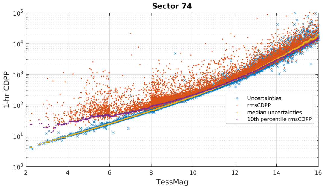
Figure 6: 1-hour CDPP. The red points are the RMS CDPP measurements for the 11774 light curves from Sector 74 plotted as a function of TESS magnitude. The blue x's are the uncertainties, scaled to 1-hour timescale. The purple curve is a moving 10th percentile of the RMS CDPP measurements, and the gold curve is a moving median of the 1-hr uncertainties.
