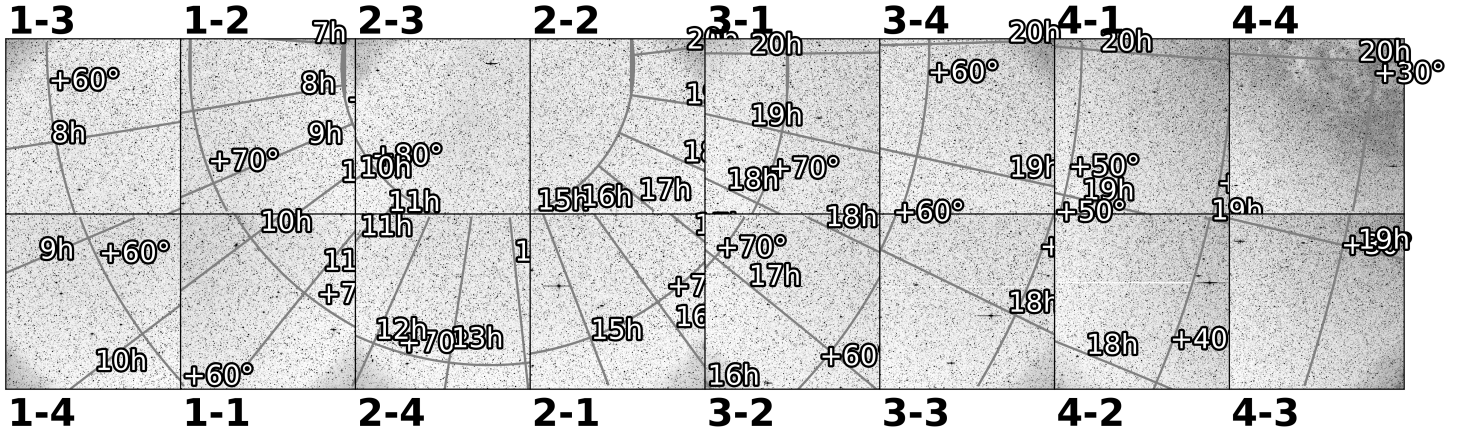
Figure 1: Grayscale TESS image for each camera and CCD (format camera#-CCD#) as labeled next to each panel. Inverse scaling (dark represents higher image flux and light represents lower flux) is used. Grid lines represent RA and Declination.
