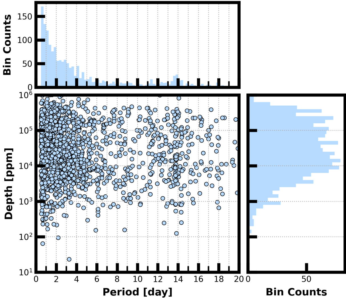
Figure 8: Lower Left Panel: Transit depth as a function of orbital period for the 1976 TCEs identified for the Sector 74 search. For enhanced visibility of long period detections, TCEs with orbital period < 0.5 days are not shown. Reported depth comes from the DV limb-darkened transit fit depth when available, and the DV trapezoid model fit depth when not available. Top Panel: Orbital period distribution of the TCEs shown in the lower left panel. Right Panel: Transit depth distribution for the TCEs shown in the lower left panel.
