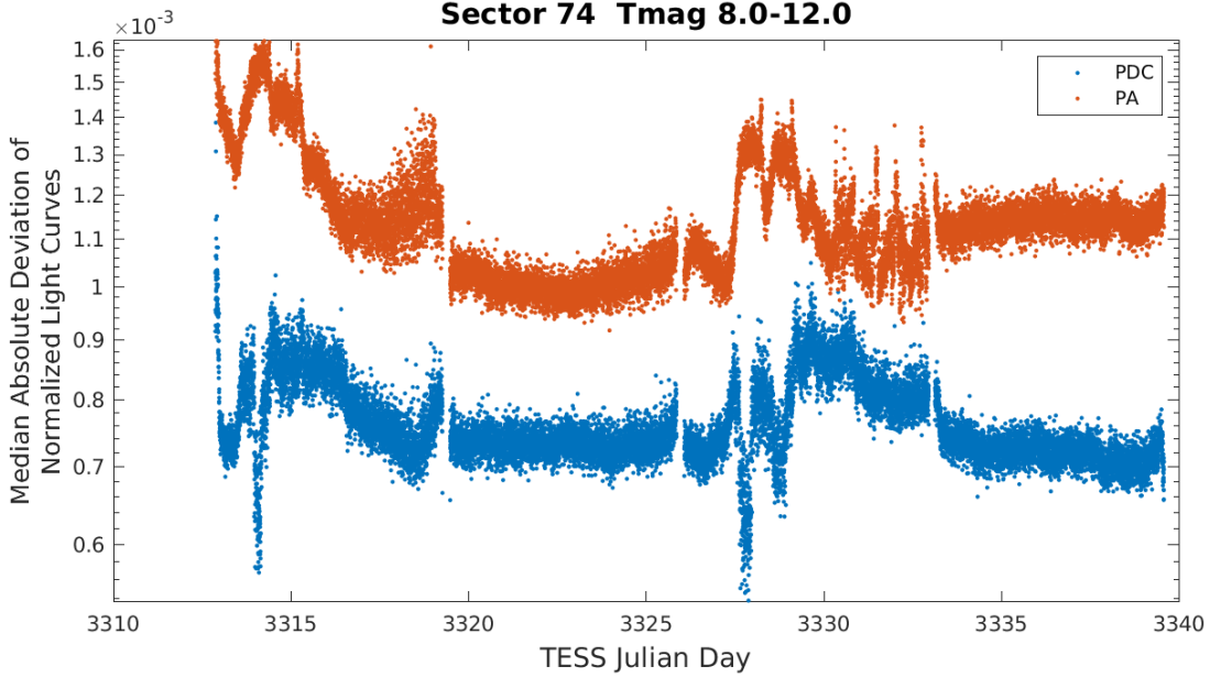
Figure 5: Median absolute deviation (MAD) for the two-minute cadence data from Sector 74, showing the performance of the cotrending after identifying Manual Exclude data quality flags. The MAD is calculated in each cadence across stars with flux variations less than 1% for both the PA (red) and PDC (blue) light curves, where each light curve is normalized by its median flux value. The scatter in the PA light curves is much higher than that for the PDC light curves, and the outliers in the PA light curves are largely absent from the PDC light curves due to the use of the anomaly flags.
