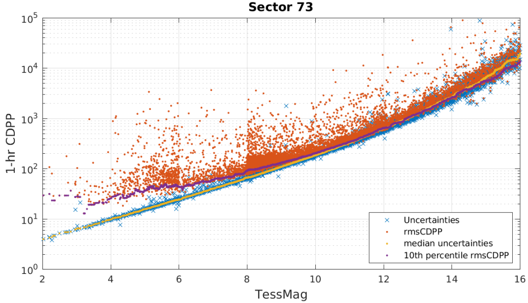
Figure 6: 1-hour CDPP. The red points are the RMS CDPP measurements for the 10648 light curves from Sector 73 plotted as a function of TESS magnitude. The blue x’s are the uncertainties, scaled to 1-hour timescale. The purple curve is a moving 10th percentile of the RMS CDPP measurements, and the gold curve is a moving median of the 1-hr uncertainties.
