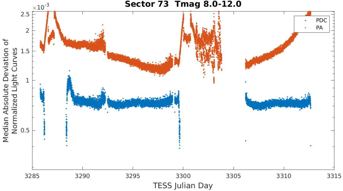
Figure 5: Median absolute deviation (MAD) for the two-minute cadence data from Sector 73, showing the performance of the cotrending after identifying Manual Exclude data quality flags. The MAD is calculated in each cadence across stars with flux variations less than 1% for both the PA (red) and PDC (blue) light curves, where each light curve is normalized by its median flux value. The scatter in the PA light curves is much higher than that for the PDC light curves, and the outliers in the PA light curves are largely absent from the PDC light curves due to the use of the anomaly flags.
