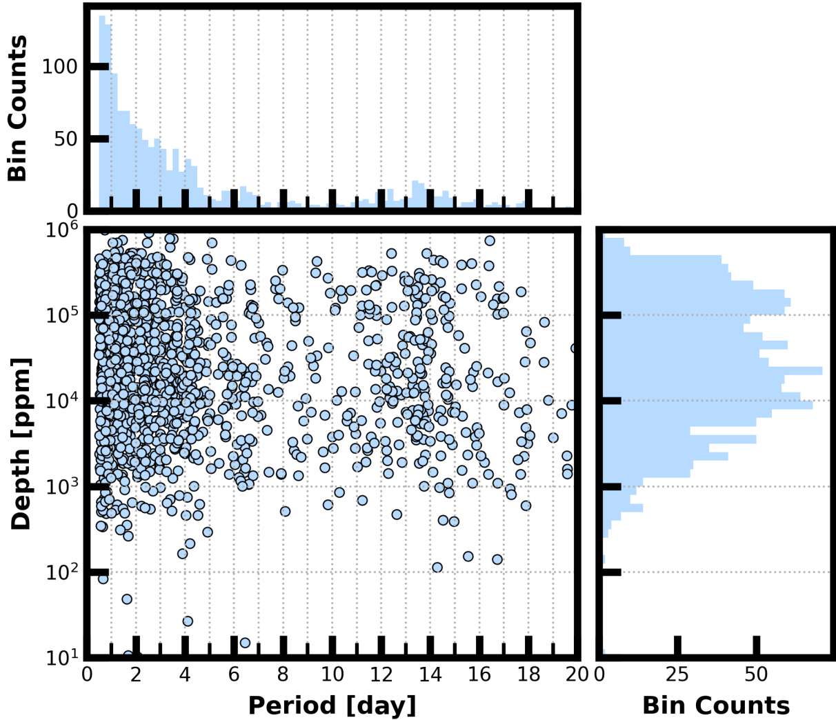
Figure 8: Lower Left Panel: Transit depth as a function of orbital period for the 1632 TCEs identified for the Sector 73 search. For enhanced visibility of long period detections, TCEs with orbital period < 0.5 days are not shown. Reported depth comes from the DV limb-darkened transit fit depth when available, and the DV trapezoid model fit depth when not available. Top Panel: Orbital period distribution of the TCEs shown in the lower left panel. Right Panel: Transit depth distribution for the TCEs shown in the lower left panel.
