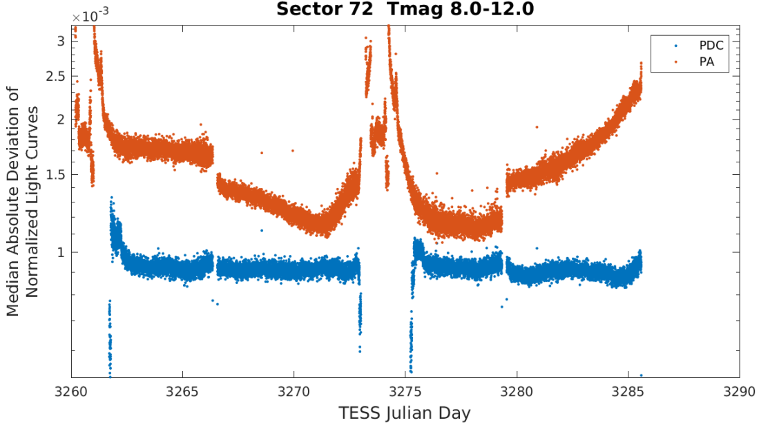
Figure 5: Median absolute deviation (MAD) for the two-minute cadence data from Sector 72, showing the performance of the cotrending after identifying Manual Exclude data quality flags. The MAD is calculated in each cadence across stars with flux variations less than 1% for both the PA (red) and PDC (blue) light curves, where each light curve is normalized by its median flux value. The scatter in the PA light curves is much higher than that for the PDC light curves, and the outliers in the PA light curves are largely absent from the PDC light curves due to the use of the anomaly flags.
