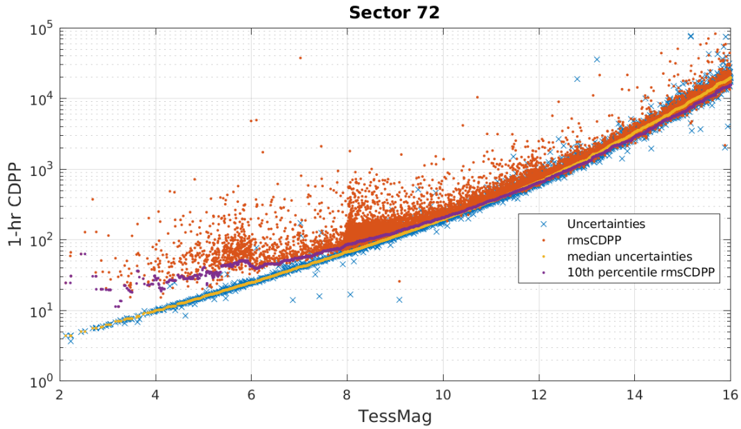
Figure 6: 1-hour CDPP. The red points are the RMS CDPP measurements for the 12098 light curves from Sector 72 plotted as a function of TESS magnitude. The blue x's are the uncertainties, scaled to 1-hour timescale. The purple curve is a moving 10th percentile of the RMS CDPP measurements, and the gold curve is a moving median of the 1-hr uncertainties.
