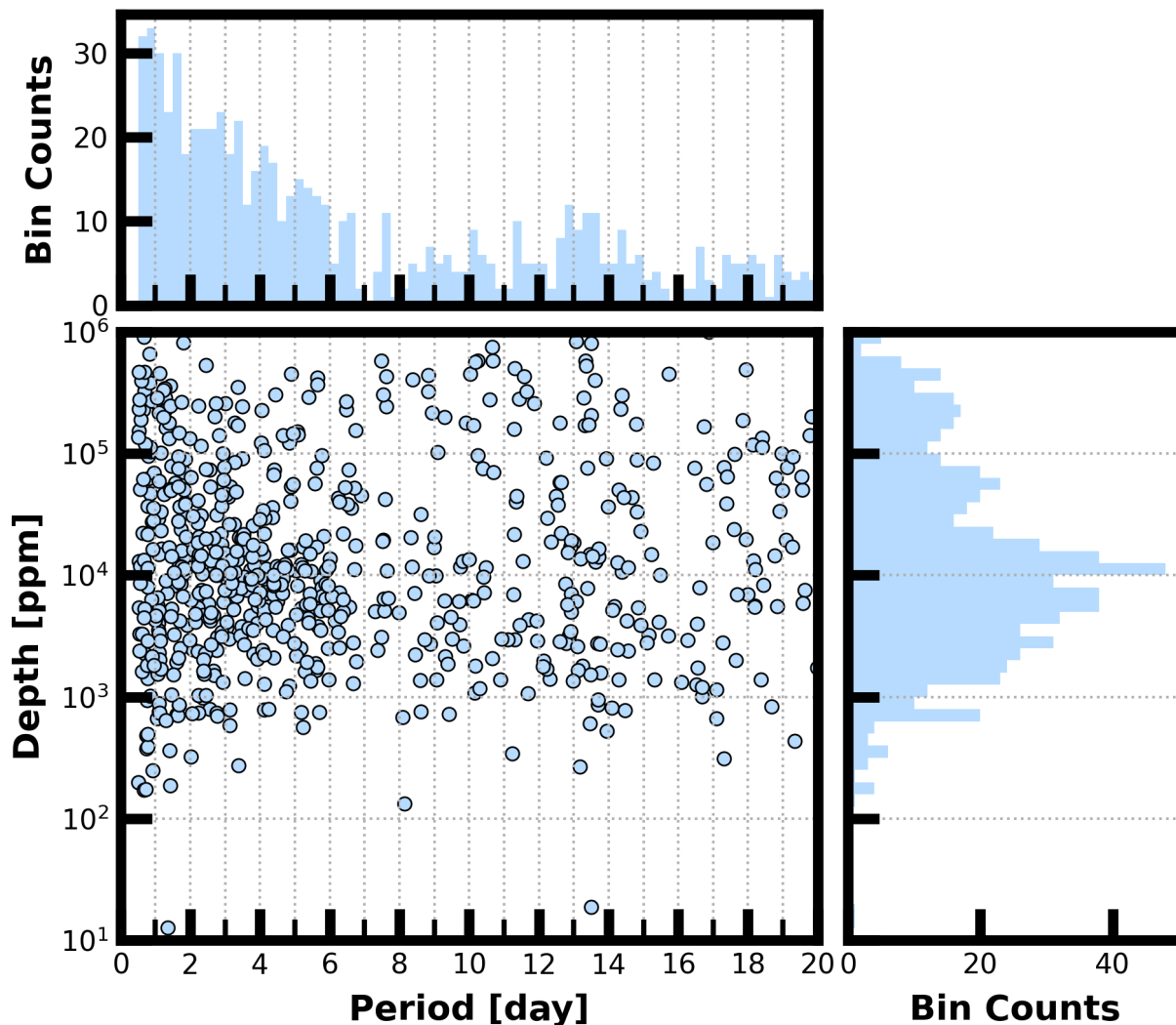
Figure 8: Lower Left Panel: Transit depth as a function of orbital period for the 846 TCEs identified for the Sector 72 search. For enhanced visibility of long period detections, TCEs with orbital period <0.5 days are not shown. Reported depth comes from the DV limb-darkened transit fit depth when available, and the DV trapezoid model fit depth when not available. Top Panel: Orbital period distribution of the TCEs shown in the lower left panel. Right Panel: Transit depth distribution for the TCEs shown in the lower left panel.
