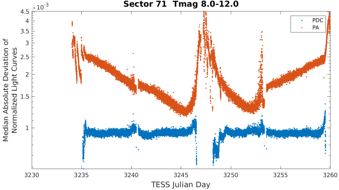
Figure 6: Median absolute deviation (MAD) for the two-minute cadence data from Sector 71, showing the performance of the cotrending after identifying Manual Exclude data quality flags. The MAD is calculated in each cadence across stars with flux variations less than 1% for both the PA (red) and PDC (blue) light curves, where each light curve is normalized by its median flux value. The scatter in the PA light curves is much higher than that for the PDC light curves, and the outliers in the PA light curves are largely absent from the PDC light curves due to the use of the anomaly flags.
