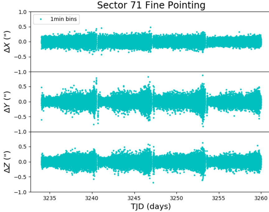
Figure 3: The delta-quaternions from each camera have been converted to spacecraft frame, binned to 1 minute. Long-term trends (such as those caused by differential velocity aberration) have also been removed. The \Delta X/\Delta Y directions represent offsets along the detectors’ rows/columns, while the \Delta Z direction represents spacecraft roll.
