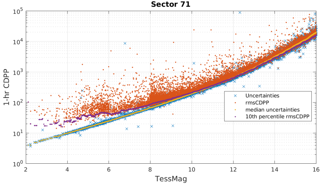
Figure 7: 1-hour CDPP. The red points are the RMS CDPP measurements for the 12965 light curves from Sector 71 plotted as a function of TESS magnitude. The blue x’s are the uncertainties, scaled to 1-hour timescale. The purple curve is a moving 10th percentile of the RMS CDPP measurements, and the gold curve is a moving median of the 1-hr uncertainties.
