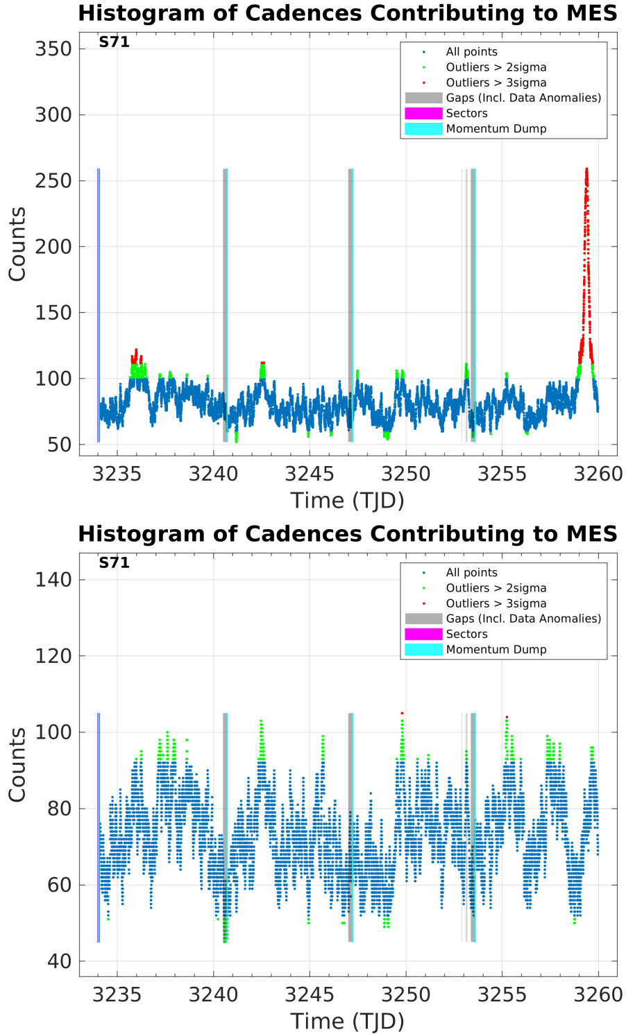
Figure 8: Top panel: Number of TCEs at a given cadence exhibiting a transit signal, based on an initial run of TPS. Any isolated peaks are caused by single events that result in spurious TCEs. These peaks were used to define de-emphasis weights that suppress problematic epochs for the transit detection statistics in a second iteration of TPS. Bottom panel: Results from the second run of TPS.
