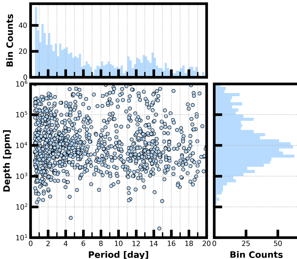
Figure 9: Lower Left Panel: Transit depth as a function of orbital period for the 1186 TCEs identified for the Sector 71 search. For enhanced visibility of long period detections, TCEs with orbital period <0.5 days are not shown. Reported depth comes from the DV limb-darkened transit fit depth when available, and the DV trapezoid model fit depth when not available. Top Panel: Orbital period distribution of the TCEs shown in the lower left panel. Right Panel: Transit depth distribution for the TCEs shown in the lower left panel.
