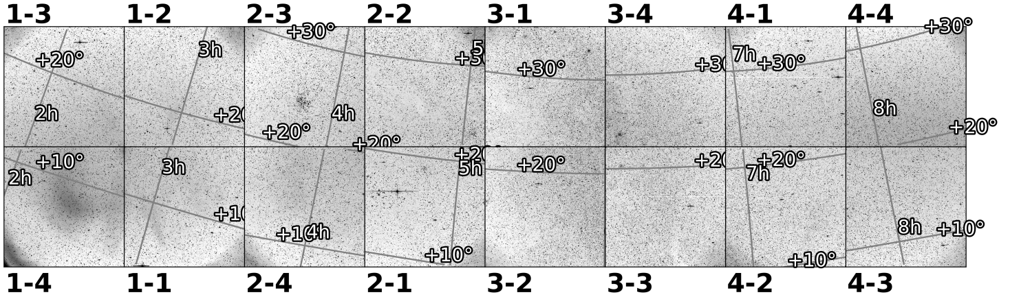
Figure 2: Grayscale TESS image for each camera and CCD (format camera#-CCD#) as labeled next to each panel. The image data for Camera 1 and CCD 4 is shown before Jupiter enters the field of view. Inverse scaling (dark represents higher image flux and light represents lower flux) is used. Grid lines represent RA and Declination.
