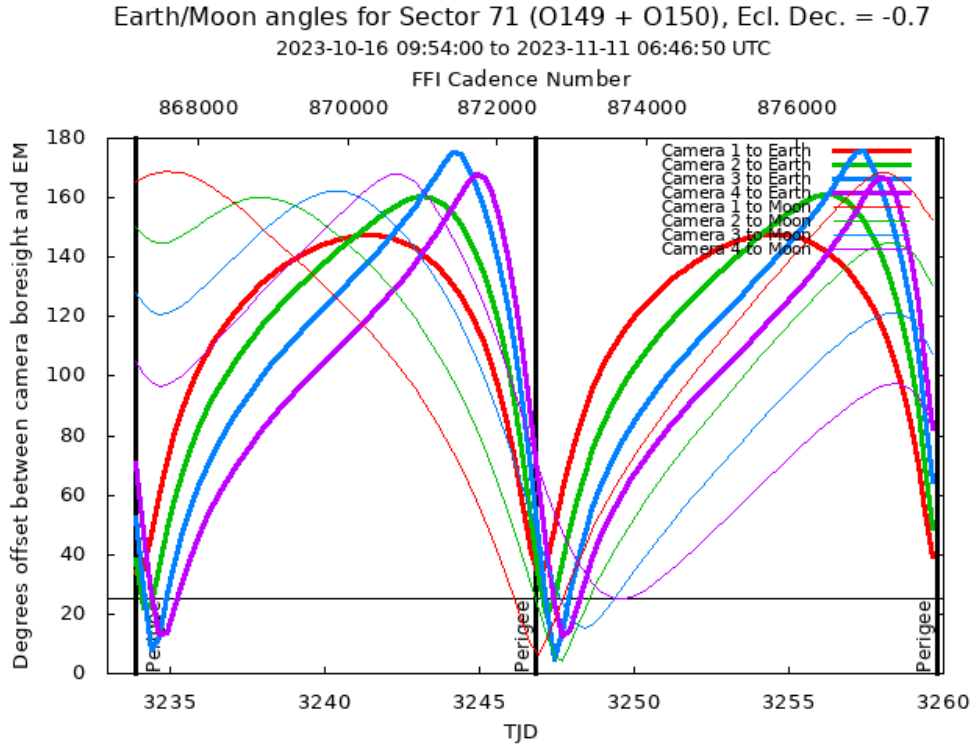
Figure 5: Angle between the four camera boresights and the Earth/Moon as a function of time. When the Earth is within \sim 25^\circ of a camera’s boresight, transiting planet searches may be compromised by high levels of scattered light. At larger angles, up to \sim 35^\circ , scattered light patterns and complicated structures may be visible. At yet larger angles, low level patchy features may be visible. Scattered light from the Moon is generally only noticeable below \sim 35^\circ . This figure can be used to identify periods affected by scattered light and the relative contributions of the Earth and Moon to the background. However, the background intensity and locations of scattered light features depend on additional factors, such as the Earth/Moon azimuth and distance from the spacecraft.
