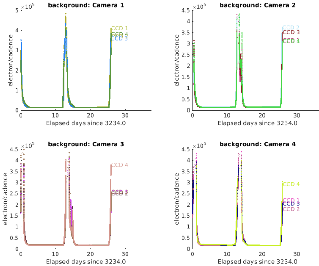
Figure 4: Median background flux across all targets on a given CCD in each camera. The changes are caused by variations in the orientation and distance of the Earth and Moon.
