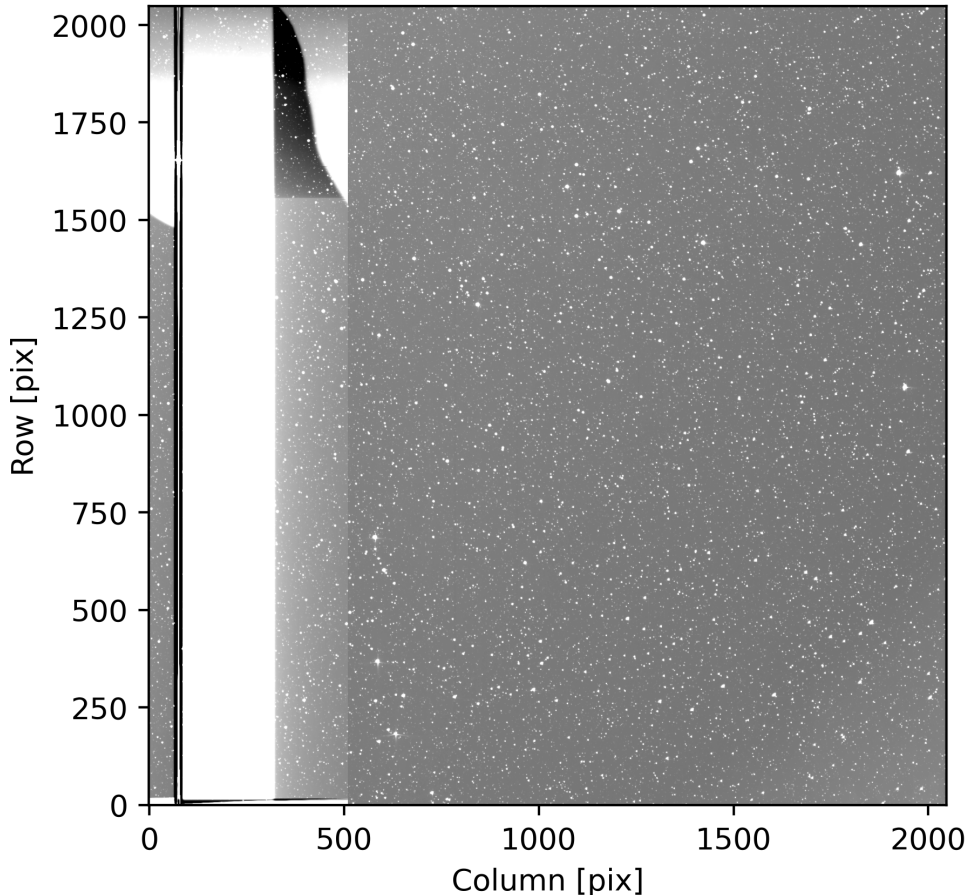
Figure 1: Grayscale TESS FFI for Camera 1, CCD 4 showing the impact of Jupiter on the calibrated image. The calibration is unreliable for the slice A readout columns (Columns 45 – 556), and targets on this slice have unreliable photometry. The color scaling is such that white represents a higher flux and a darker gray represents a lower flux.
