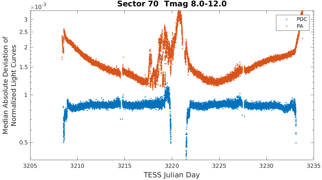
Figure 5: Median absolute deviation (MAD) for the two-minute cadence data from Sector 70, showing the performance of the cotrending after identifying Manual Exclude data quality flags. The MAD is calculated in each cadence across stars with flux variations less than 1% for both the PA (red) and PDC (blue) light curves, where each light curve is normalized by its median flux value. The scatter in the PA light curves is much higher than that for the PDC light curves, and the outliers in the PA light curves are largely absent from the PDC light curves due to the use of the anomaly flags.
