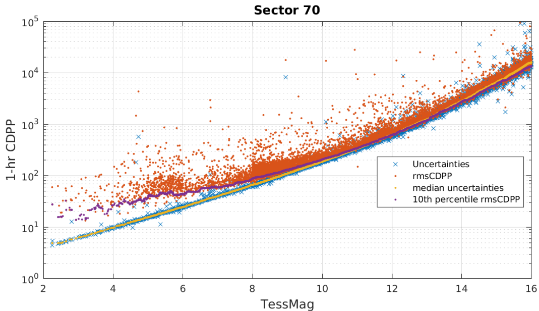
Figure 6: 1-hour CDPP. The red points are the RMS CDPP measurements for the 12797 light curves from Sector 70 plotted as a function of TESS magnitude. The blue x's are the uncertainties, scaled to 1-hour timescale. The purple curve is a moving 10th percentile of the RMS CDPP measurements, and the gold curve is a moving median of the 1-hr uncertainties.
