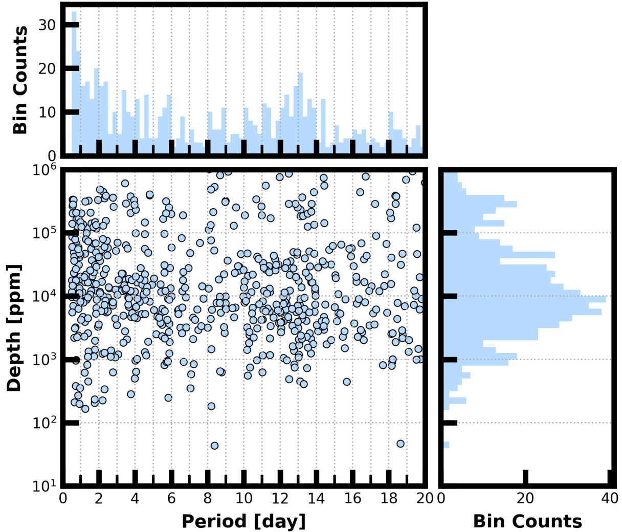
Figure 8: Lower Left Panel: Transit depth as a function of orbital period for the 783 TCEs identified for the Sector 70 search. For enhanced visibility of long period detections, TCEs with orbital period < 0.5 days are not shown. Reported depth comes from the DV limb-darkened transit fit depth when available, and the DV trapezoid model fit depth when not available. Top Panel: Orbital period distribution of the TCEs shown in the lower left panel. Right Panel: Transit depth distribution for the TCEs shown in the lower left panel.
