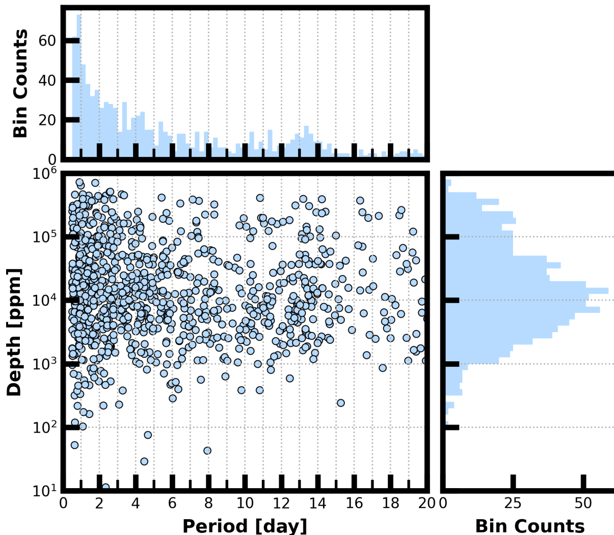
Figure 8: Lower Left Panel: Transit depth as a function of orbital period for the 1215 TCEs identified for the Sector 69 search. For enhanced visibility of long period detections, TCEs with orbital period <0.5 days are not shown. Reported depth comes from the DV limb-darkened transit fit depth when available, and the DV trapezoid model fit depth when not available. Top Panel: Orbital period distribution of the TCEs shown in the lower left panel. Right Panel: Transit depth distribution for the TCEs shown in the lower left panel.
