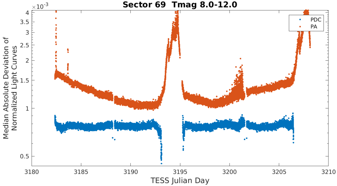
Figure 5: Median absolute deviation (MAD) for the two-minute cadence data from Sector 69, showing the performance of the cotrending after identifying Manual Exclude data quality flags. The MAD is calculated in each cadence across stars with flux variations less than 1% for both the PA (red) and PDC (blue) light curves, where each light curve is normalized by its median flux value. The scatter in the PA light curves is much higher than that for the PDC light curves, and the outliers in the PA light curves are largely absent from the PDC light curves due to the use of the anomaly flags.
