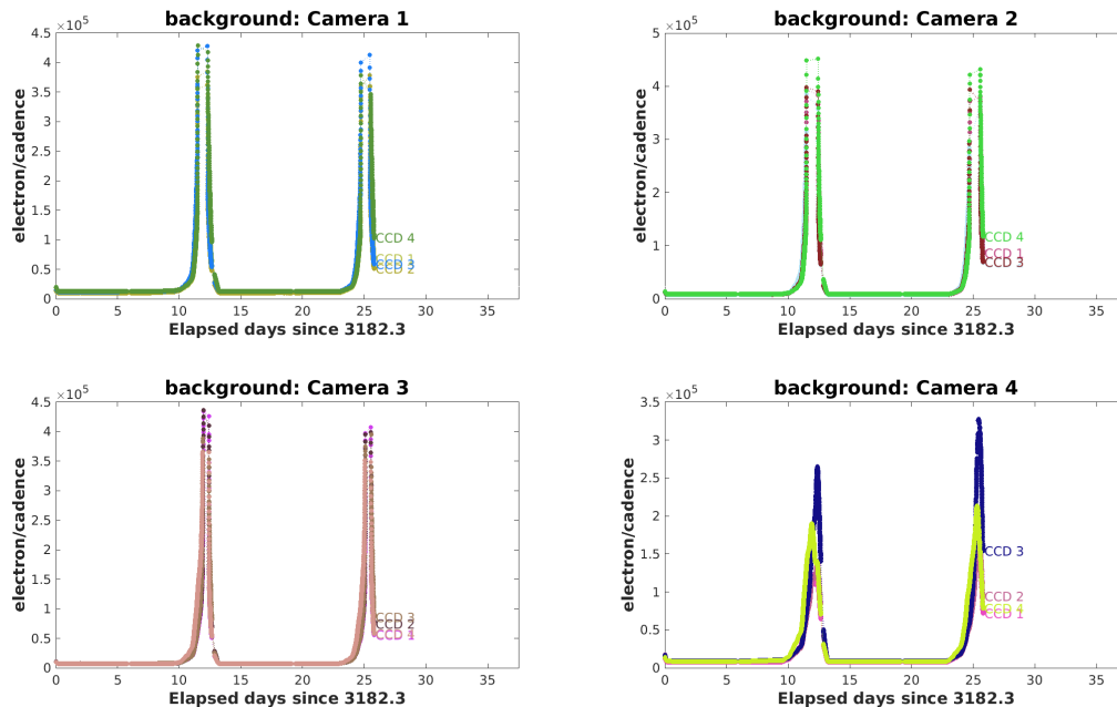
Figure 3: Median background flux across all targets on a given CCD in each camera. The changes are caused by variations in the orientation and distance of the Earth and Moon.
