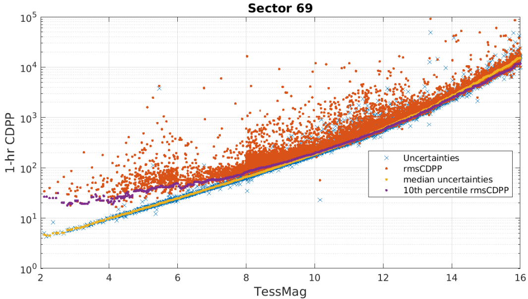
Figure 6: 1-hour CDPP. The red points are the RMS CDPP measurements for the 10541 light curves from Sector 69 plotted as a function of TESS magnitude. The blue x's are the uncertainties, scaled to 1-hour timescale. The purple curve is a moving 10th percentile of the RMS CDPP measurements, and the gold curve is a moving median of the 1-hr uncertainties.
