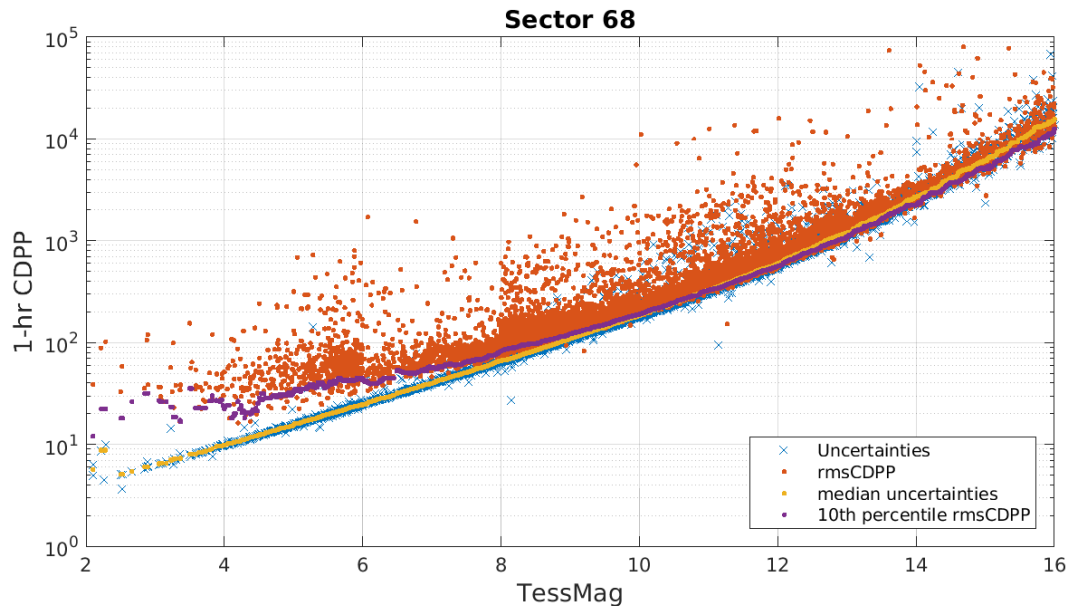
Figure 6: 1-hour CDPP. The red points are the RMS CDPP measurements for the 10573 light curves from Sector 68 plotted as a function of TESS magnitude. The blue x's are the uncertainties, scaled to 1-hour timescale. The purple curve is a moving 10th percentile of the RMS CDPP measurements, and the gold curve is a moving median of the 1-hr uncertainties.
