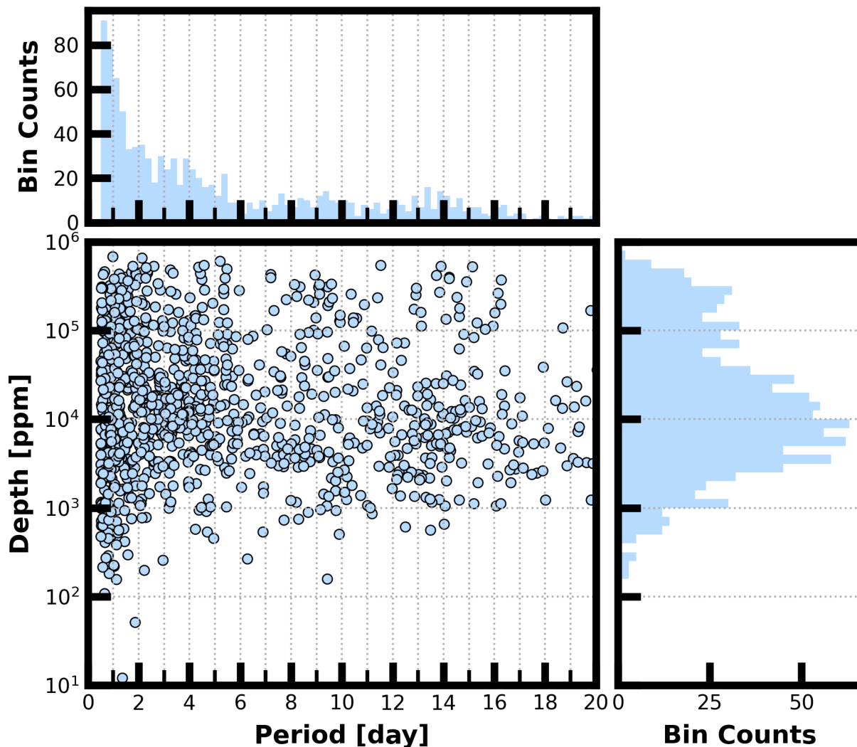
Figure 8: Lower Left Panel: Transit depth as a function of orbital period for the 1373 TCEs identified for the Sector 68 search. For enhanced visibility of long period detections, TCEs with orbital period < 0.5 days are not shown. Reported depth comes from the DV limb-darkened transit fit depth when available, and the DV trapezoid model fit depth when not available. Top Panel: Orbital period distribution of the TCEs shown in the lower left panel. Right Panel: Transit depth distribution for the TCEs shown in the lower left panel.
