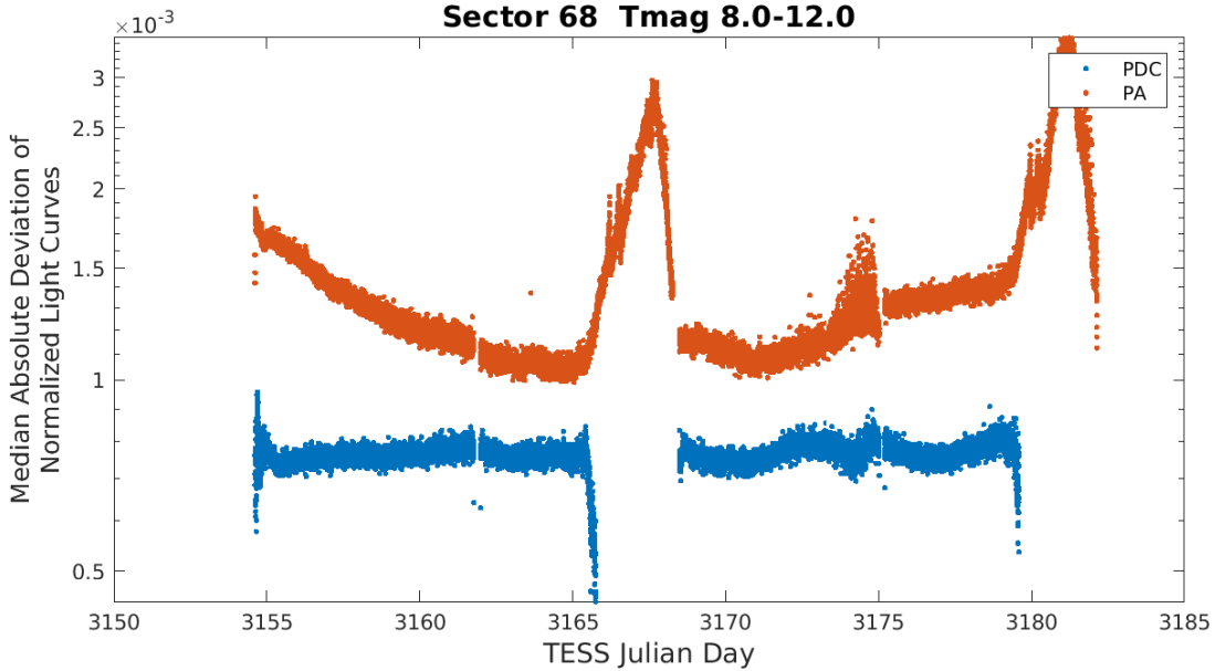
Figure 5: Median absolute deviation (MAD) for the two-minute cadence data from Sector 68, showing the performance of the cotrending after identifying Manual Exclude data quality flags. The MAD is calculated in each cadence across stars with flux variations less than 1% for both the PA (red) and PDC (blue) light curves, where each light curve is normalized by its median flux value. The scatter in the PA light curves is much higher than that for the PDC light curves, and the outliers in the PA light curves are largely absent from the PDC light curves due to the use of the anomaly flags.
