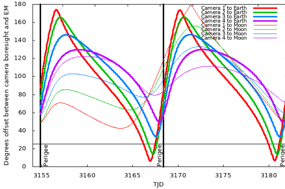
Figure 4: Angle between the four camera boresights and the Earth/Moon as a function of time. When the Earth is within \sim 25^\circ of a camera’s boresight, transiting planet searches may be compromised by high levels of scattered light. At larger angles, up to \sim 35^\circ , scattered light patterns and complicated structures may be visible. At yet larger angles, low level patchy features may be visible. Scattered light from the Moon is generally only noticeable below \sim 35^\circ . This figure can be used to identify periods affected by scattered light and the relative contributions of the Earth and Moon to the background. However, the background intensity and locations of scattered light features depend on additional factors, such as the Earth/Moon azimuth and distance from the spacecraft.
