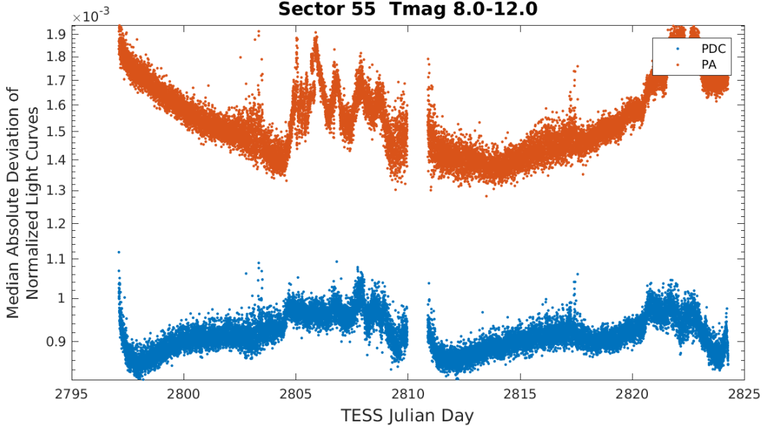
Figure 4: Median absolute deviation (MAD) for the two-minute cadence data from Sector 55, showing the performance of the cotrending after identifying Manual Exclude data quality flags. The MAD is calculated in each cadence across stars with flux variations less than 1% for both the PA (red) and PDC (blue) light curves, where each light curve is normalized by its median flux value. The scatter in the PA light curves is much higher than that for the PDC light curves, and the outliers in the PA light curves are largely absent from the PDC light curves due to the use of the anomaly flags.
