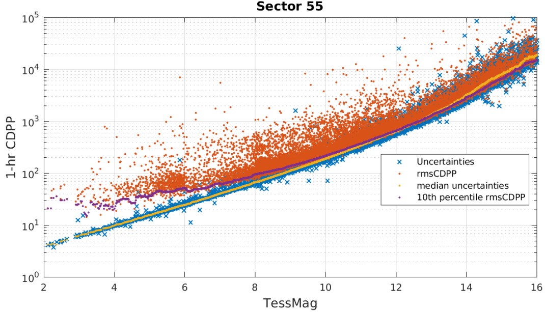
Figure 6: 1-hour CDPP. The red points are the RMS CDPP measurements for the 19996 light curves from Sector 55 plotted as a function of TESS magnitude. The blue x’s are the uncertainties, scaled to 1-hour timescale. The purple curve is a moving 10th percentile of the RMS CDPP measurements, and the gold curve is a moving median of the 1-hr uncertainties.
