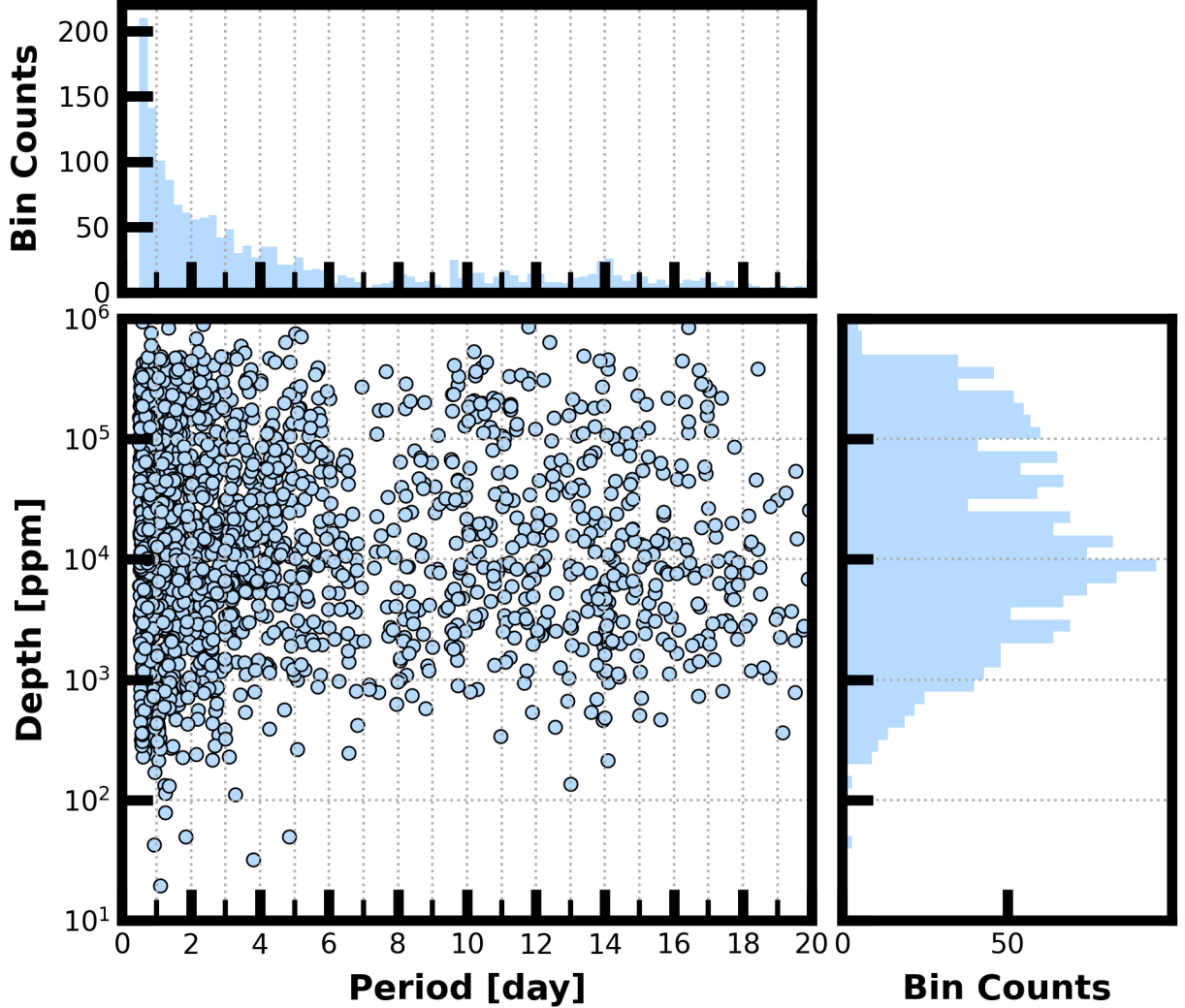
Figure 8: Lower Left Panel: Transit depth as a function of orbital period for the 2294 TCEs identified for the Sector 55 search. For enhanced visibility of long period detections, TCEs with orbital period < 0.5 days are not shown. Reported depth comes from the DV limb-darkened transit fit depth when available, and the DV trapezoid model fit depth when not available. Top Panel: Orbital period distribution of the TCEs shown in the lower left panel. Right Panel: Transit depth distribution for the TCEs shown in the lower left panel.
