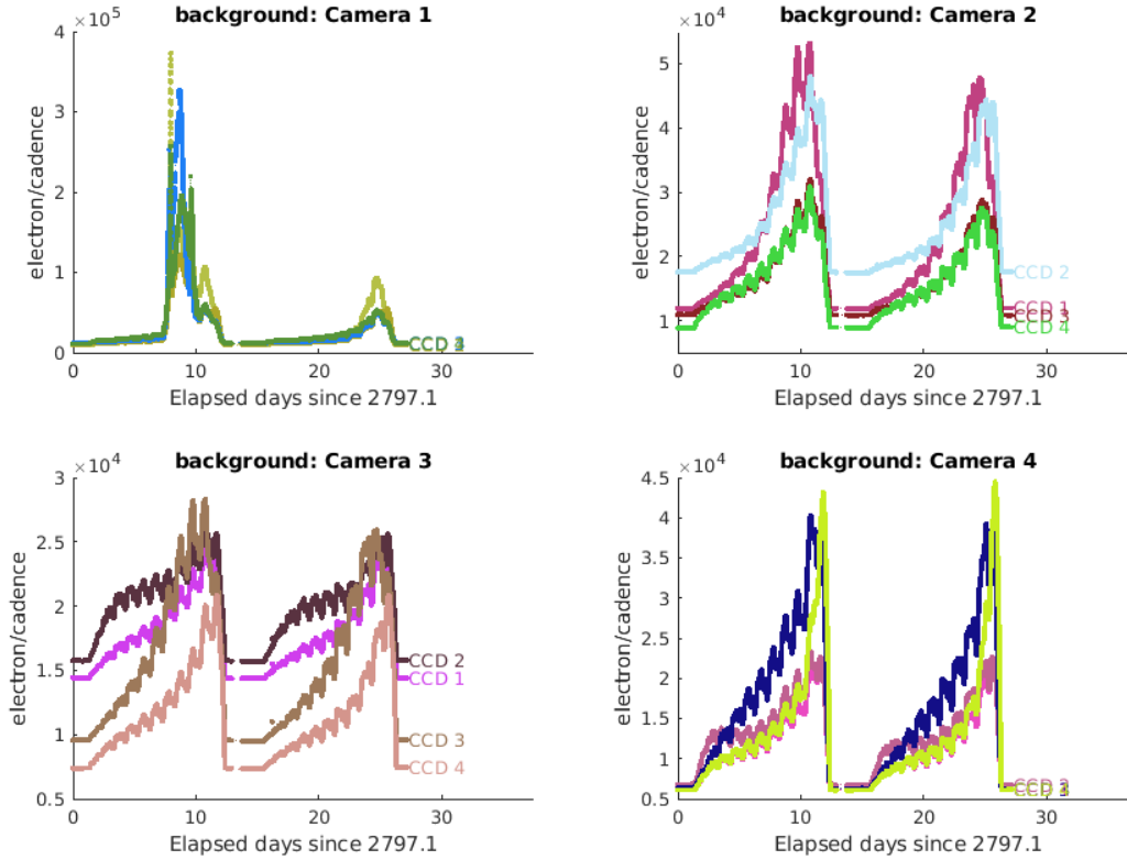
Figure 2: Median background flux across all targets on a given CCD in each camera. The changes are caused by variations in the orientation and distance of the Earth and Moon. In Sector 55, the Earth and Moon pass through the camera fields of view, saturating the detectors.
