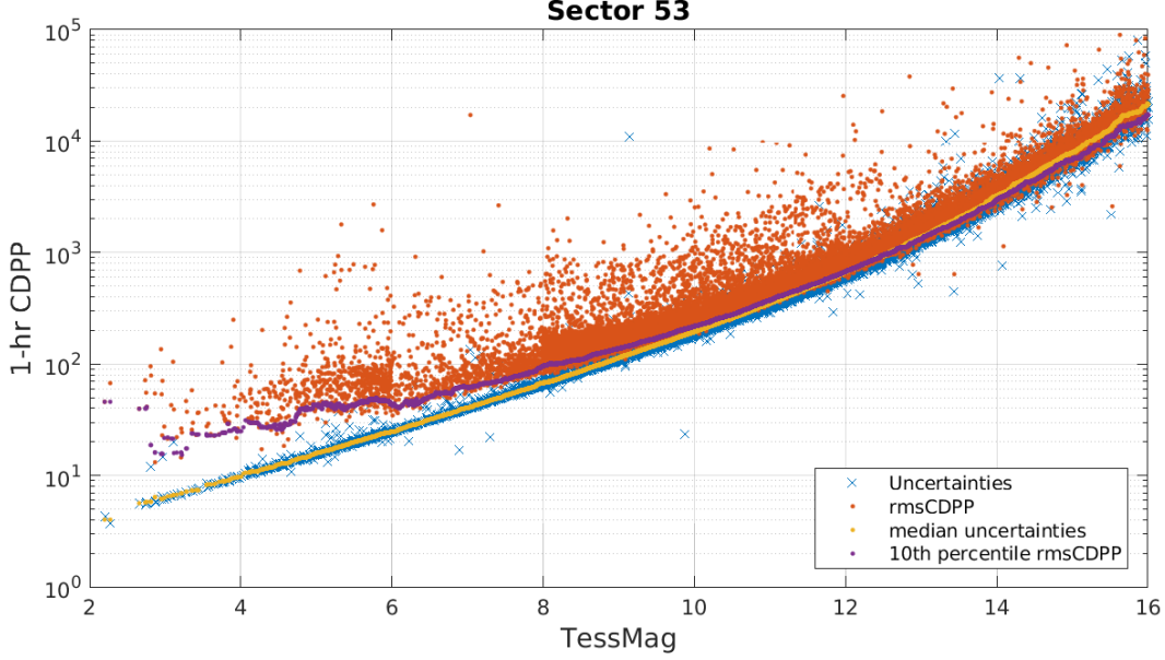
Figure 6: 1-hour CDPP. The red points are the RMS CDPP measurements for the 19995 light curves from Sector 53 plotted as a function of TESS magnitude. The blue x’s are the uncertainties, scaled to 1-hour timescale. The purple curve is a moving 10th percentile of the RMS CDPP measurements, and the gold curve is a moving median of the 1-hr uncertainties.
