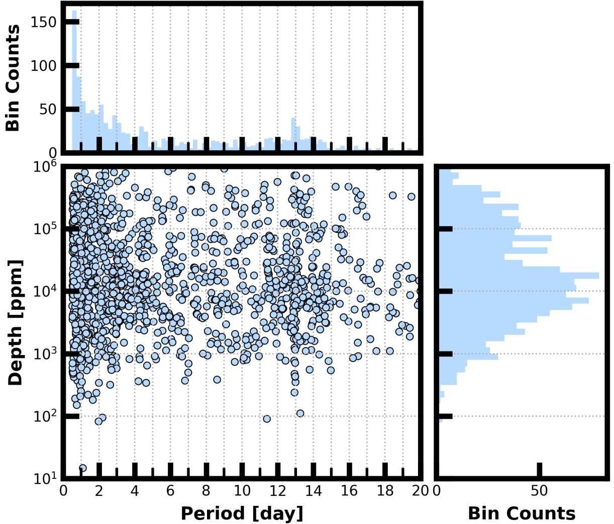
Figure 8: Lower Left Panel: Transit depth as a function of orbital period for the 1789 TCEs identified for the Sector 53 search. For enhanced visibility of long period detections, TCEs with orbital period < 0.5 days are not shown. Reported depth comes from the DV limb-darkened transit fit depth when available, and the DV trapezoid model fit depth when not available. Top Panel: Orbital period distribution of the TCEs shown in the lower left panel. Right Panel: Transit depth distribution for the TCEs shown in the lower left panel.
