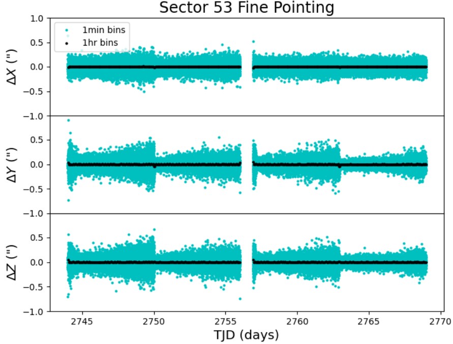
Figure 1: The delta-quaternions from each camera have been converted to spacecraft frame, binned to 1 minute and 1 hour. The figure for Sector 53 only shows quaternions from Camera 4. Long-term trends (such as those caused by differential velocity aberration) have also been removed. The \Delta X/\Delta Y directions represent offsets along the detectors' rows/columns, while the \Delta Z direction represents spacecraft roll.
