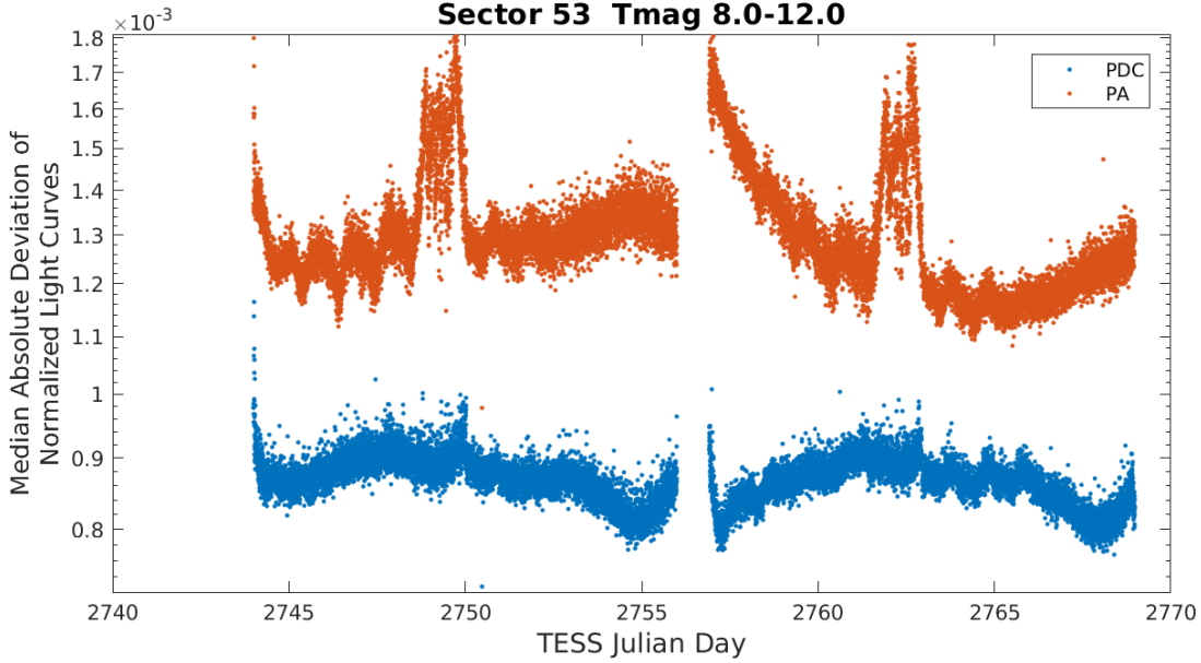
Figure 4: Median absolute deviation (MAD) for the two-minute cadence data from Sector 53, showing the performance of the cotrending after identifying Manual Exclude data quality flags. The MAD is calculated in each cadence across stars with flux variations less than 1% for both the PA (red) and PDC (blue) light curves, where each light curve is normalized by its median flux value. The scatter in the PA light curves is much higher than that for the PDC light curves, and the outliers in the PA light curves are largely absent from the PDC light curves due to the use of the anomaly flags.
