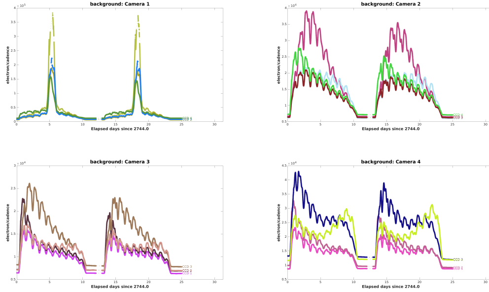
Figure 2: Median background flux across all targets on a given CCD in each camera. The changes are caused by variations in the orientation and distance of the Earth and Moon. In Sector 53, the Earth and Moon pass through the camera fields of view, saturating the detectors.
