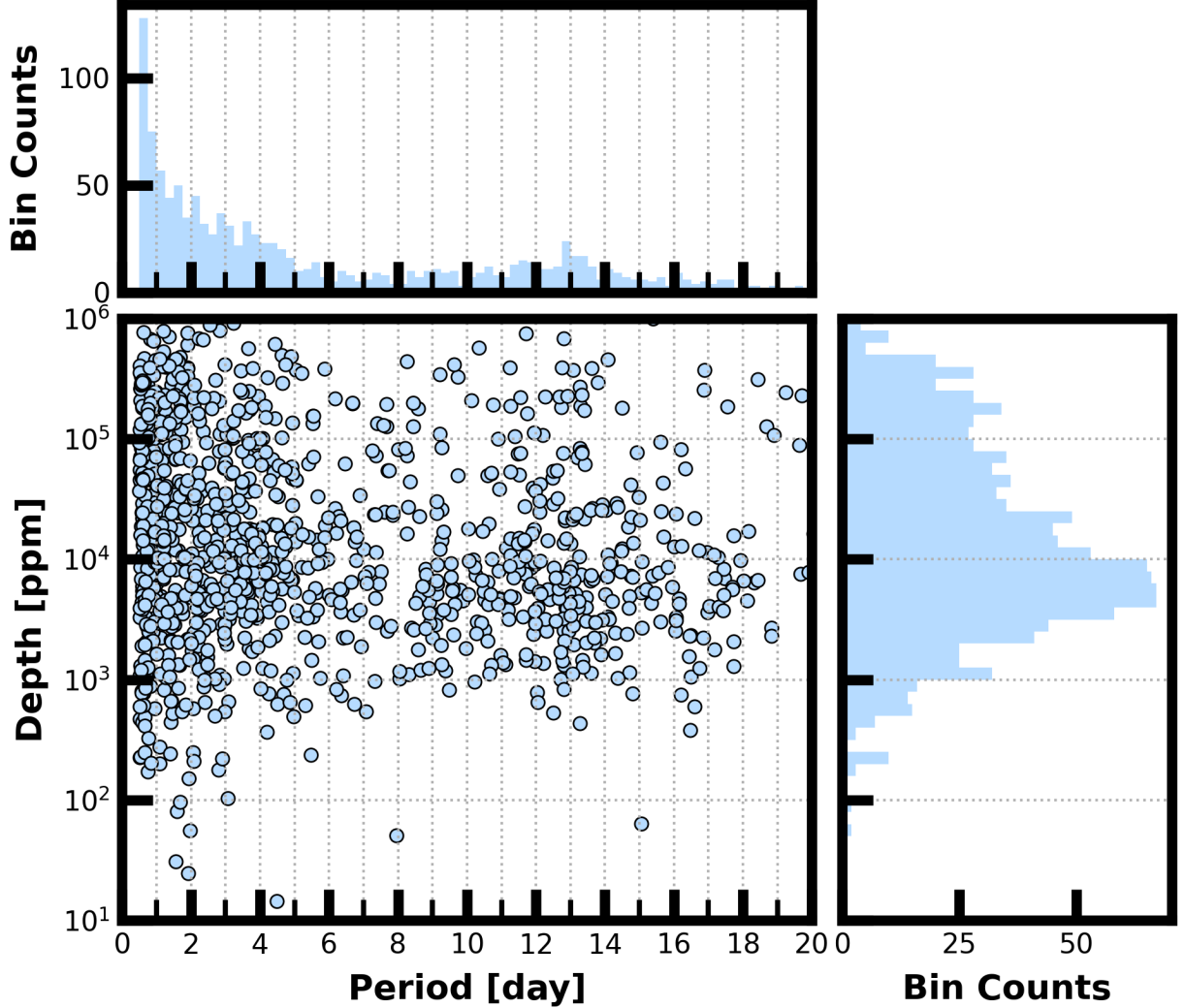
Figure 8: Lower Left Panel: Transit depth as a function of orbital period for the 1522 TCEs identified for the Sector 52 search. For enhanced visibility of long period detections, TCEs with orbital period < 0.5 days are not shown. Reported depth comes from the DV limb-darkened transit fit depth when available, and the DV trapezoid model fit depth when not available. Top Panel: Orbital period distribution of the TCEs shown in the lower left panel. Right Panel: Transit depth distribution for the TCEs shown in the lower left panel.
