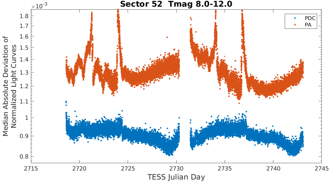
Figure 4: Median absolute deviation (MAD) for the two-minute cadence data from Sector 52, showing the performance of the cotrending after identifying Manual Exclude data quality flags. The MAD is calculated in each cadence across stars with flux variations less than 1% for both the PA (red) and PDC (blue) light curves, where each light curve is normalized by its median flux value. The scatter in the PA light curves is much higher than that for the PDC light curves, and the outliers in the PA light curves are largely absent from the PDC light curves due to the use of the anomaly flags.
