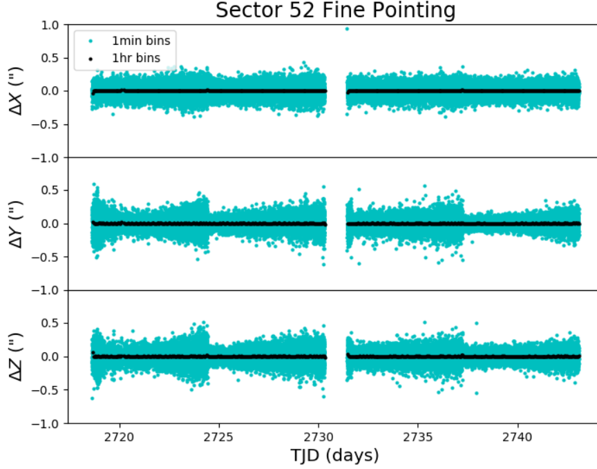
Figure 1: The delta-quaternions from each camera have been converted to spacecraft frame, binned to 1 minute and 1 hour. The figure for Sector 52 only shows quaternions from Camera 4. Long-term trends (such as those caused by differential velocity aberration) have also been removed. The \Delta X/\Delta Y directions represent offsets along the detectors’ rows/columns, while the \Delta Z direction represents spacecraft roll.
