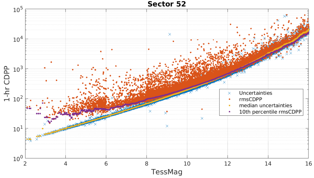
Figure 6: 1-hour CDPP. The red points are the RMS CDPP measurements for the 19996 light curves from Sector 52 plotted as a function of TESS magnitude. The blue x's are the uncertainties, scaled to 1-hour timescale. The purple curve is a moving 10th percentile of the RMS CDPP measurements, and the gold curve is a moving median of the 1-hr uncertainties.
