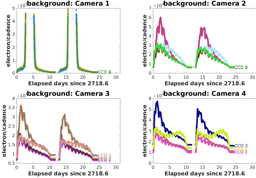
Figure 2: Median background flux across all targets on a given CCD in each camera. The changes are caused by variations in the orientation and distance of the Earth and Moon. In Sector 52, the Earth and Moon pass through the camera fields of view, saturating the detectors.
