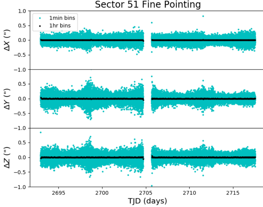
Figure 1: The delta-quaternions from each camera have been converted to spacecraft frame, binned to 1 minute and 1 hour. The figure for Sector 51 only shows quaternions from Camera 4. Long-term trends (such as those caused by differential velocity aberration) have also been removed. The \Delta X/\Delta Y directions represent offsets along the detectors' rows/columns, while the \Delta Z direction represents spacecraft roll.
