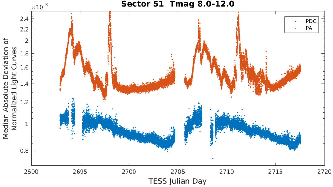
Figure 4: Median absolute deviation (MAD) for the two-minute cadence data from Sector 51, showing the performance of the cotrending after identifying Manual Exclude data quality flags. The MAD is calculated in each cadence across stars with flux variations less than 1% for both the PA (red) and PDC (blue) light curves, where each light curve is normalized by its median flux value. The scatter in the PA light curves is much higher than that for the PDC light curves, and the outliers in the PA light curves are largely absent from the PDC light curves due to the use of the anomaly flags.
