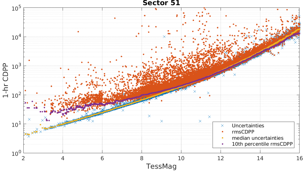
Figure 6: 1-hour CDPP. The red points are the RMS CDPP measurements for the 19997 light curves from Sector 51 plotted as a function of TESS magnitude. The blue x’s are the uncertainties, scaled to 1-hour timescale. The purple curve is a moving 10th percentile of the RMS CDPP measurements, and the gold curve is a moving median of the 1-hr uncertainties.
