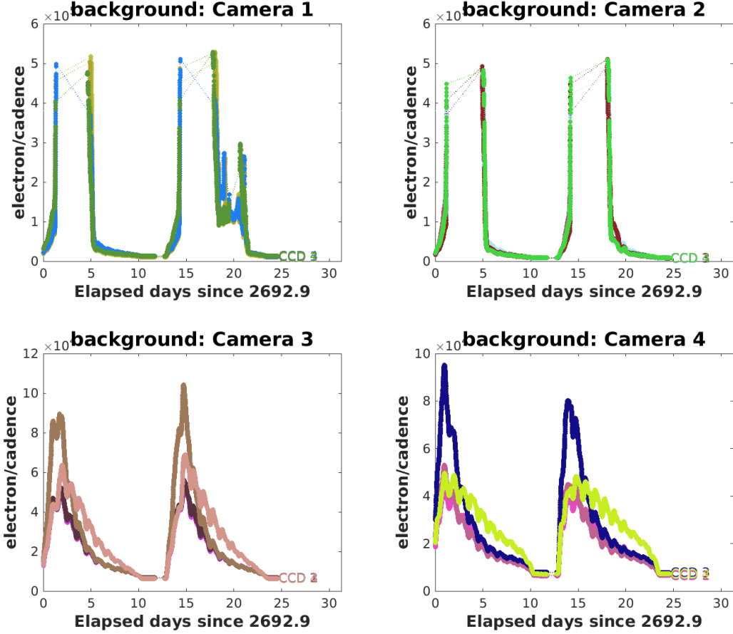
Figure 2: Median background flux across all targets on a given CCD in each camera. The changes are caused by variations in the orientation and distance of the Earth and Moon. In Sector 51, the Earth and Moon pass through the camera fields of view, saturating the detectors.
