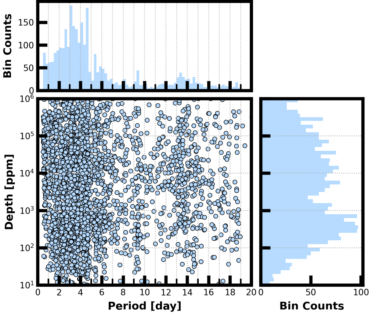
Figure 8: Lower Left Panel: Transit depth as a function of orbital period for the 3146 TCEs identified for the Sector 51 search. For enhanced visibility of long period detections, TCEs with orbital period < 0.5 days are not shown. Reported depth comes from the DV limb-darkened transit fit depth when available, and the DV trapezoid model fit depth when not available. Top Panel: Orbital period distribution of the TCEs shown in the lower left panel. Right Panel: Transit depth distribution for the TCEs shown in the lower left panel.
