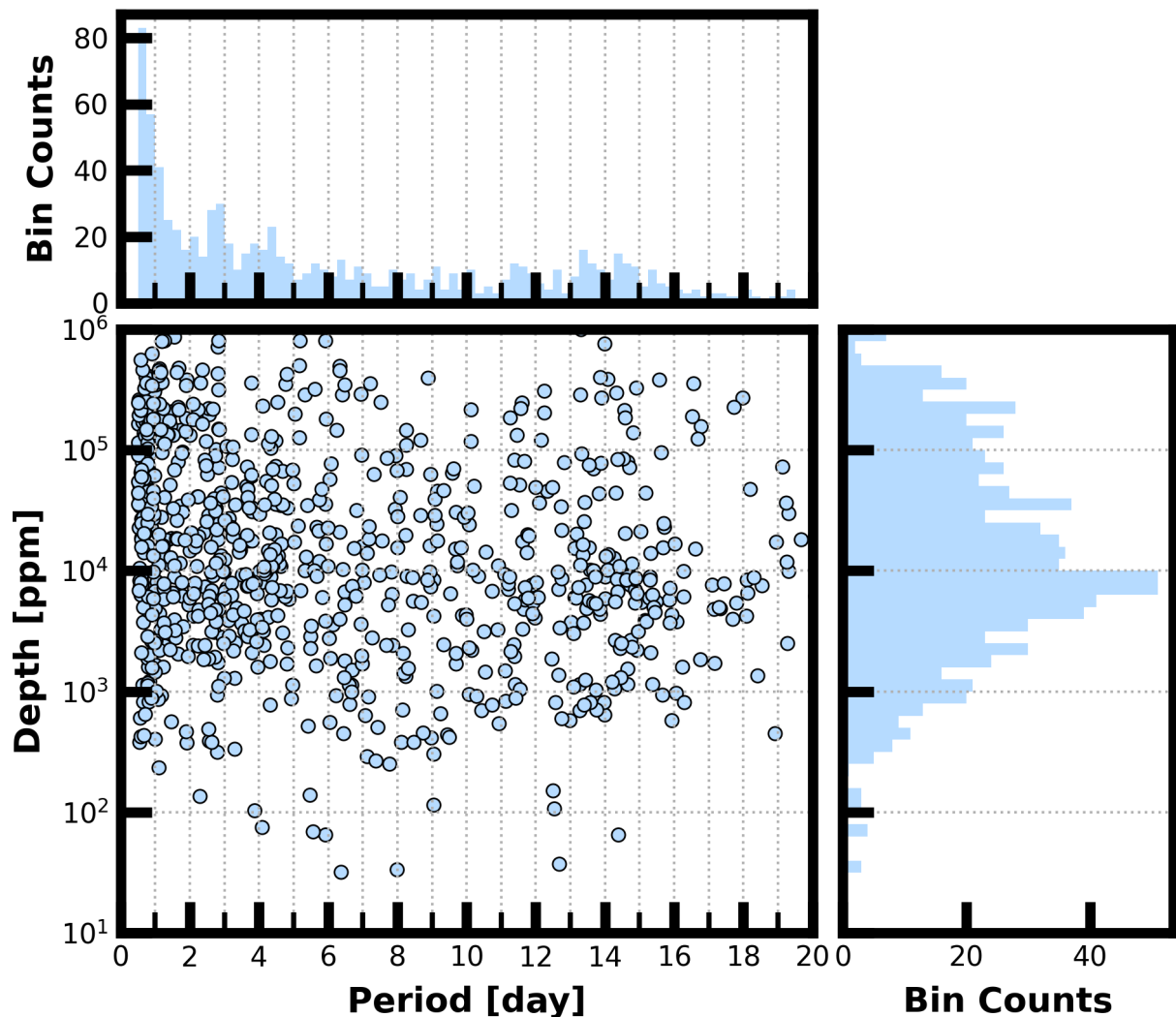
Figure 8: Lower Left Panel: Transit depth as a function of orbital period for the 1033 TCEs identified for the Sector 49 search. For enhanced visibility of long period detections, TCEs with orbital period < 0.5 days are not shown. Reported depth comes from the DV limb-darkened transit fit depth when available, and the DV trapezoid model fit depth when not available. Top Panel: Orbital period distribution of the TCEs shown in the lower left panel. Right Panel: Transit depth distribution for the TCEs shown in the lower left panel.
