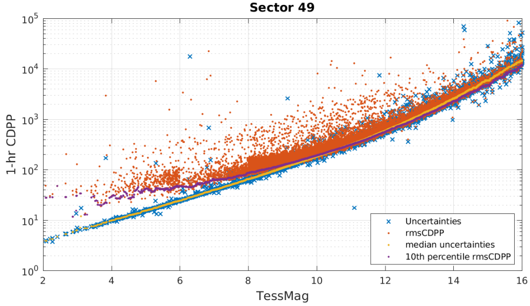
Figure 6: 1-hour CDPP. The red points are the RMS CDPP measurements for the 19999 light curves from Sector 49 plotted as a function of TESS magnitude. The blue x's are the uncertainties, scaled to 1-hour timescale. The purple curve is a moving 10th percentile of the RMS CDPP measurements, and the gold curve is a moving median of the 1-hr uncertainties.
