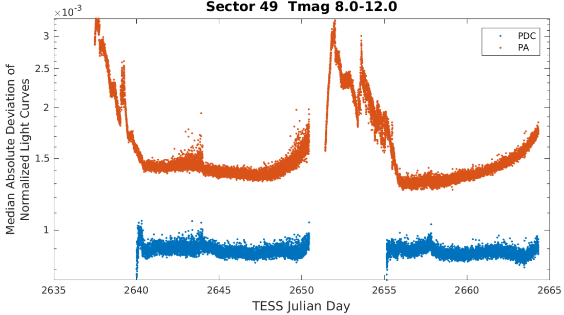
Figure 4: Median absolute deviation (MAD) for the two-minute cadence data from Sector 49, showing the performance of the cotrending after identifying Manual Exclude data quality flags. The MAD is calculated in each cadence across stars with flux variations less than 1% for both the PA (red) and PDC (blue) light curves, where each light curve is normalized by its median flux value. The scatter in the PA light curves is much higher than that for the PDC light curves, and the outliers in the PA light curves are largely absent from the PDC light curves due to the use of the anomaly flags.
