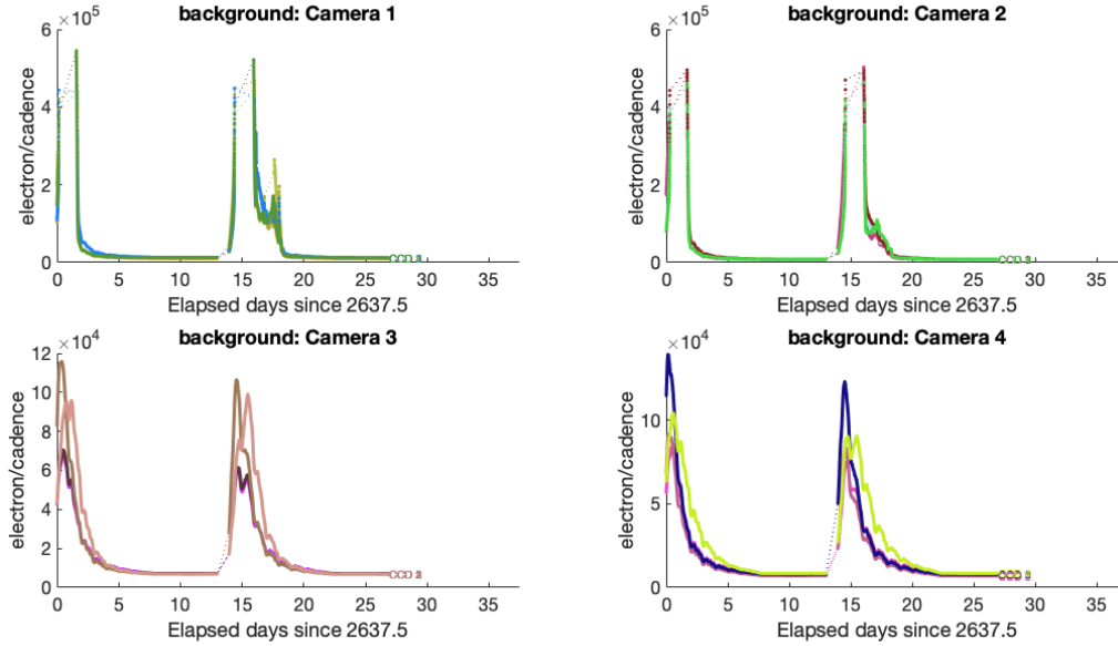
Figure 2: Median background flux across all targets on a given CCD in each camera. The changes are caused by variations in the orientation and distance of the Earth and Moon. In Sector 49, the Earth and Moon pass through the camera fields of view, saturating the detectors.
