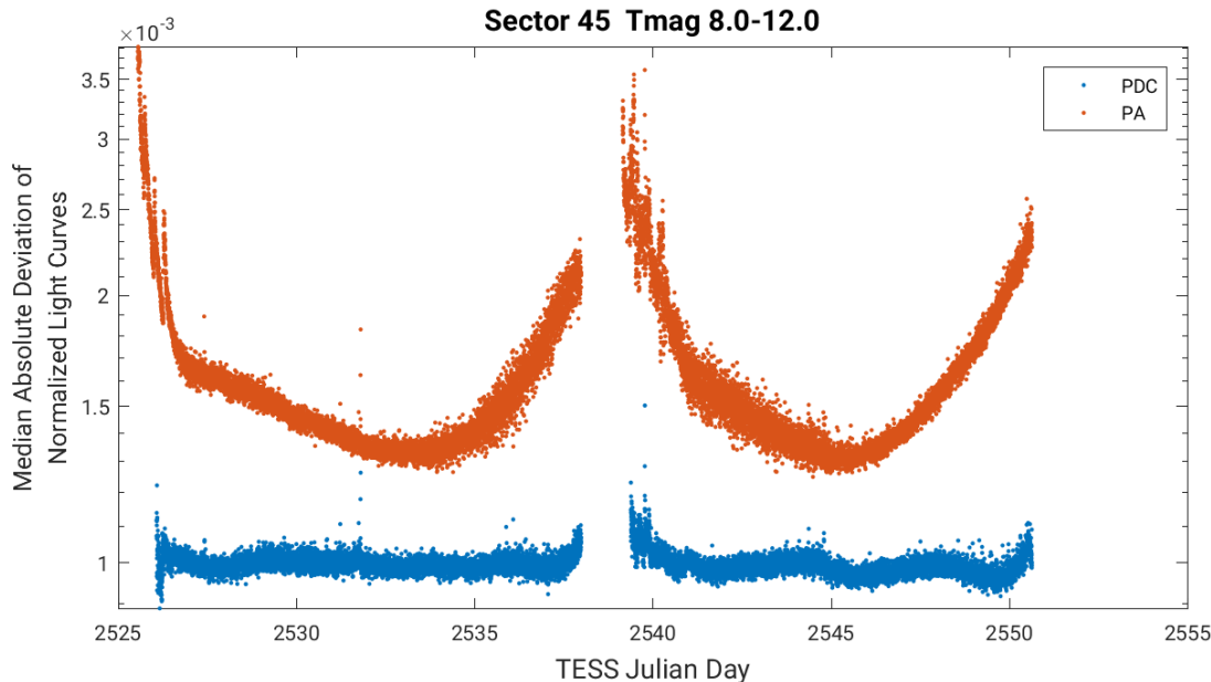
Figure 4: Median absolute deviation (MAD) for the two-minute cadence data from Sector 45, showing the performance of the cotrending after identifying Manual Exclude data quality flags. The MAD is calculated in each cadence across stars with flux variations less than 1% for both the PA (red) and PDC (blue) light curves, where each light curve is normalized by its median flux value. The scatter in the PA light curves is much higher than that for the PDC light curves, and the outliers in the PA light curves are largely absent from the PDC light curves due to the use of the anomaly flags.
