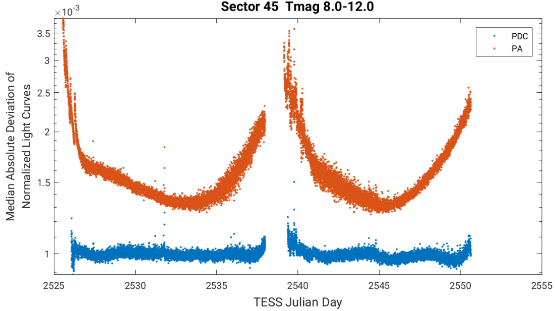
Figure 4: Median absolute deviation (MAD) for the two-minute cadence data from Sector 45, showing the performance of the cotrending after identifying Manual Exclude data quality flags. The MAD is calculated in each cadence across stars with flux variations less than 1% for both the PA (red) and PDC (blue) light curves, where each light curve is normalized by its median flux value. The scatter in the PA light curves is much higher than that for the PDC light curves, and the outliers in the PA light curves are largely absent from the PDC light curves due to the use of the anomaly flags.
