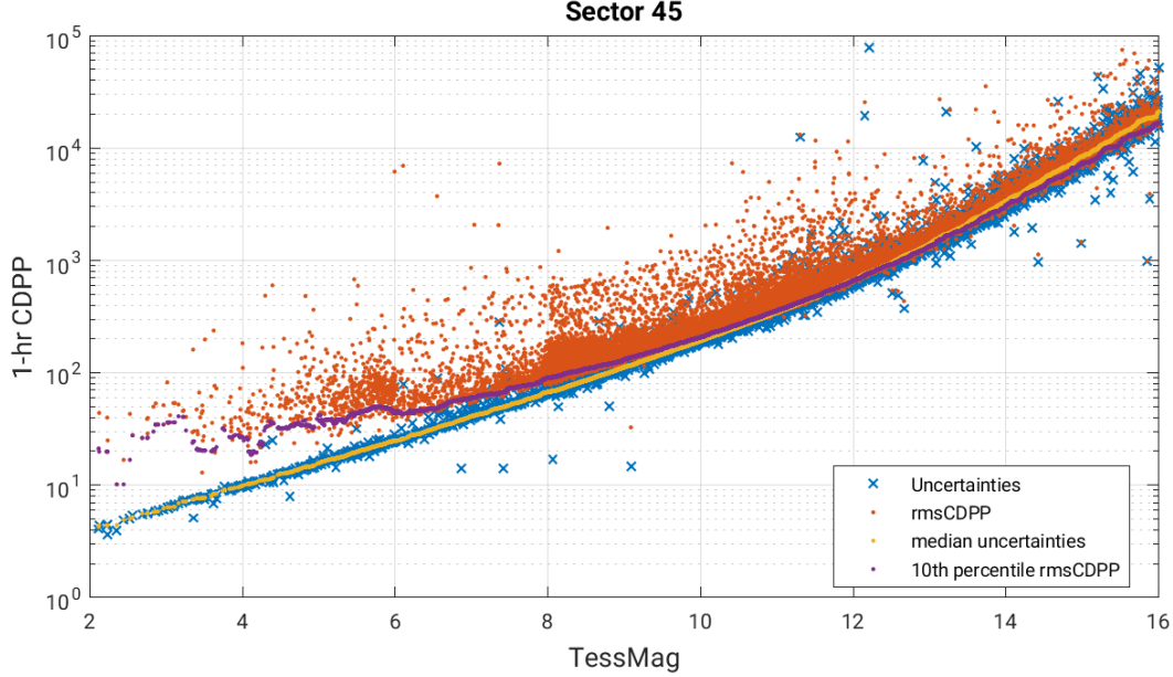
Figure 6: 1-hour CDPP. The red points are the RMS CDPP measurements for the 19996 light curves from Sector 45 plotted as a function of TESS magnitude. The blue x’s are the uncertainties, scaled to 1-hour timescale. The purple curve is a moving 10th percentile of the RMS CDPP measurements, and the gold curve is a moving median of the 1-hr uncertainties.
