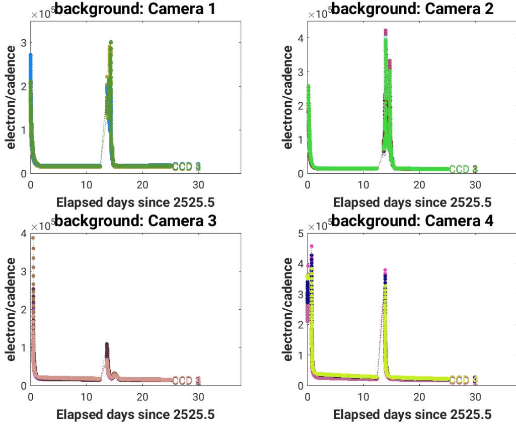
Figure 2: Median background flux across all targets on a given CCD in each camera. The changes are caused by variations in the orientation and distance of the Earth and Moon. In Sector 45, the Earth and Moon pass through the camera fields of view, saturating the detectors.
