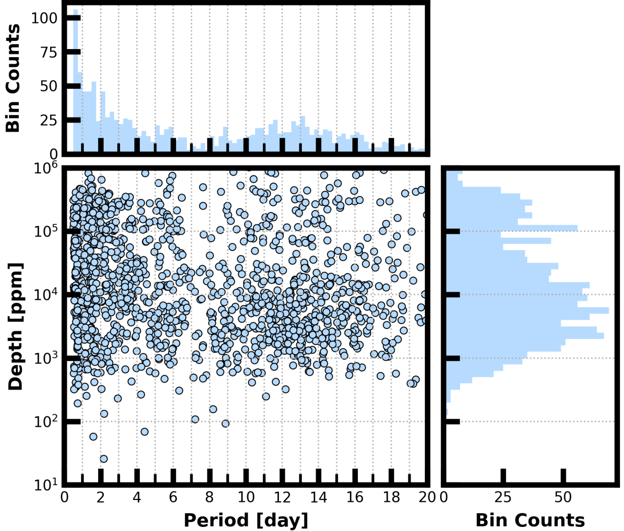
Figure 8: Lower Left Panel: Transit depth as a function of orbital period for the 1660 TCEs identified for the Sector 45 search. For enhanced visibility of long period detections, TCEs with orbital period < 0.5 days are not shown. Reported depth comes from the DV limb-darkened transit fit depth when available, and the DV trapezoid model fit depth when not available. Top Panel: Orbital period distribution of the TCEs shown in the lower left panel. Right Panel: Transit depth distribution for the TCEs shown in the lower left panel.
