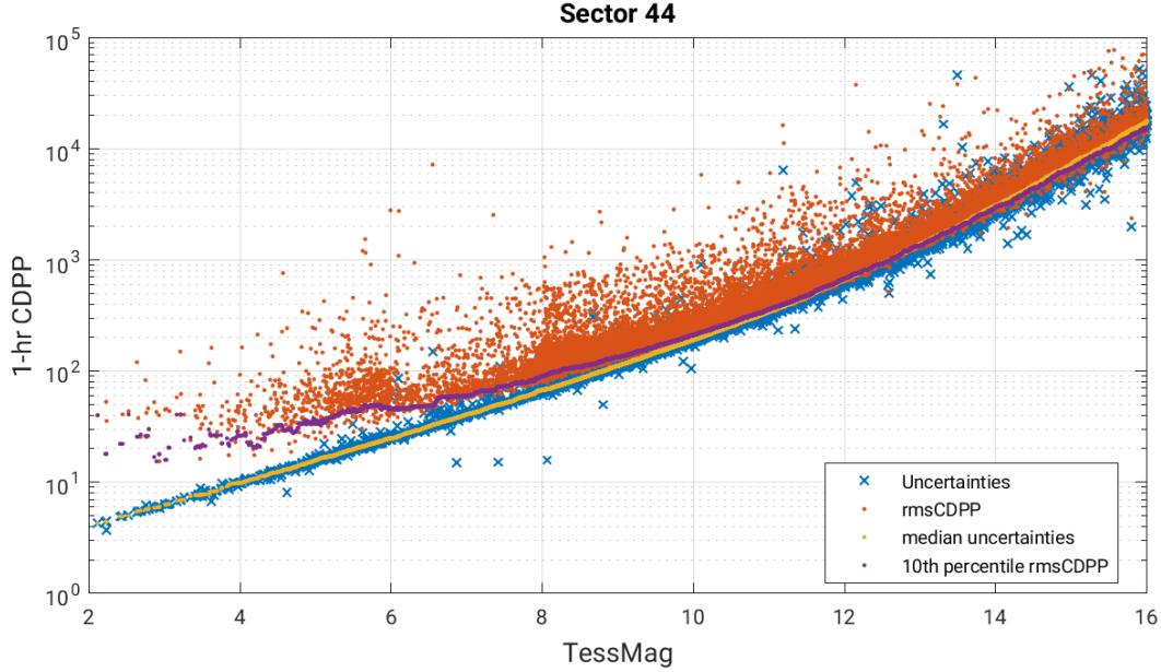
Figure 6: 1-hour CDPP. The red points are the RMS CDPP measurements for the 19994 light curves from Sector 44 plotted as a function of TESS magnitude. The blue x’s are the uncertainties, scaled to 1-hour timescale. The purple curve is a moving 10th percentile of the RMS CDPP measurements, and the gold curve is a moving median of the 1-hr uncertainties.
