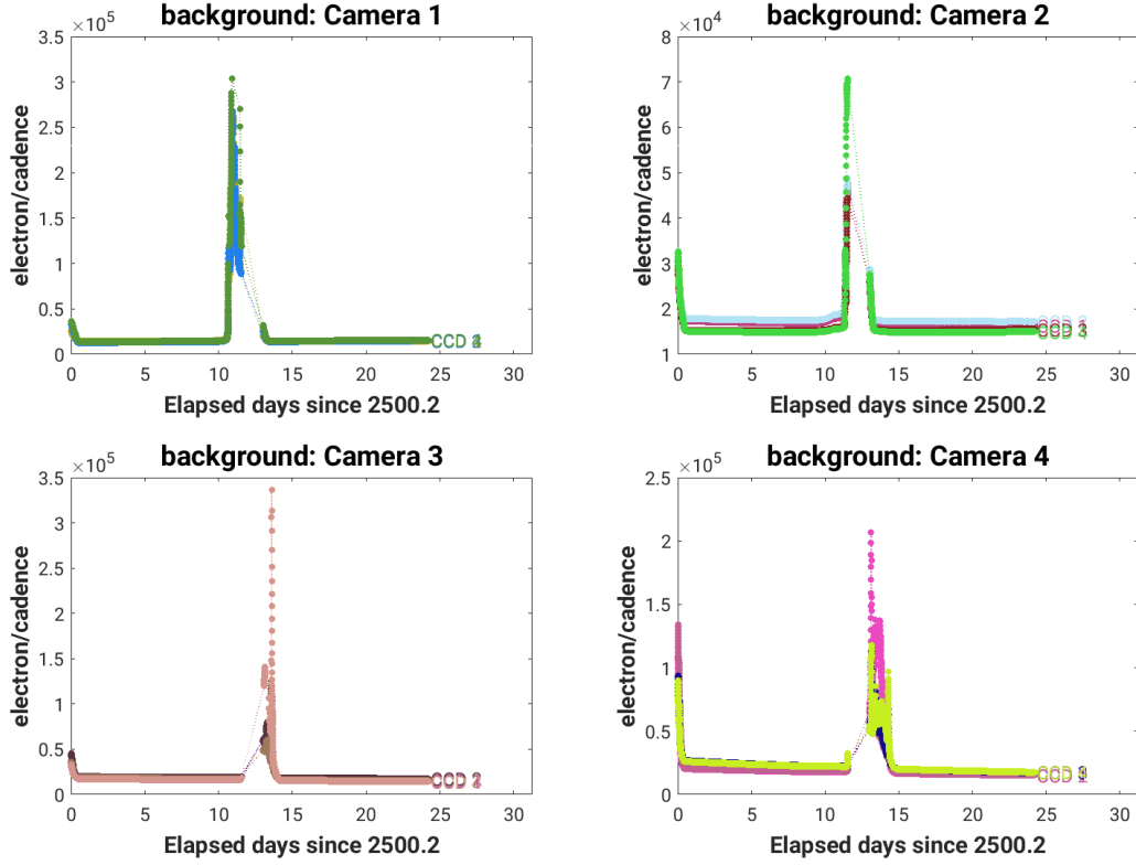
Figure 2: Median background flux across all targets on a given CCD in each camera. The changes are caused by variations in the orientation and distance of the Earth and Moon. In Sector 44, the Earth and Moon pass through the camera fields of view, saturating the detectors.
