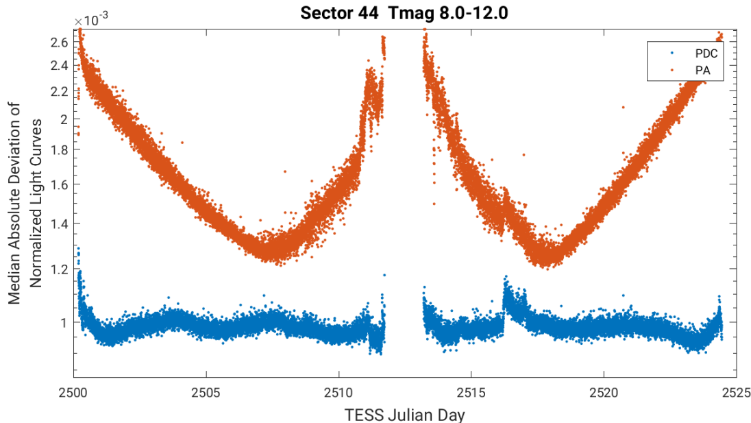
Figure 4: Median absolute deviation (MAD) for the two-minute cadence data from Sector 44, showing the performance of the cotrending after identifying Manual Exclude data quality flags. The MAD is calculated in each cadence across stars with flux variations less than 1% for both the PA (red) and PDC (blue) light curves, where each light curve is normalized by its median flux value. The scatter in the PA light curves is much higher than that for the PDC light curves, and the outliers in the PA light curves are largely absent from the PDC light curves due to the use of the anomaly flags.
