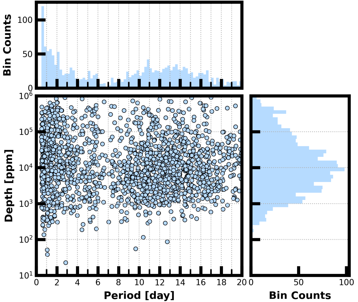
Figure 8: Lower Left Panel: Transit depth as a function of orbital period for the 2086 TCEs identified for the Sector 44 search. For enhanced visibility of long period detections, TCEs with orbital period < 0.5 days are not shown. Reported depth comes from the DV limb-darkened transit fit depth when available, and the DV trapezoid model fit depth when not available. Top Panel: Orbital period distribution of the TCEs shown in the lower left panel. Right Panel: Transit depth distribution for the TCEs shown in the lower left panel.
