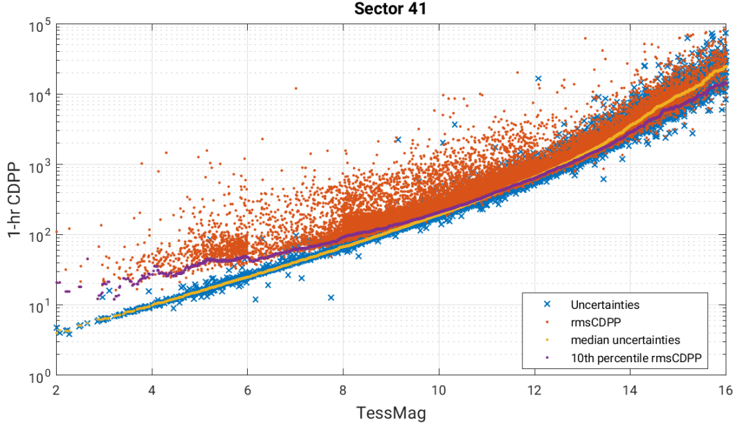
Figure 6: 1-hour CDPP. The red points are the RMS CDPP measurements for the 19996 light curves from Sector 41 plotted as a function of TESS magnitude. The blue x’s are the uncertainties, scaled to 1-hour timescale. The purple curve is a moving 10th percentile of the RMS CDPP measurements, and the gold curve is a moving median of the 1-hr uncertainties.
