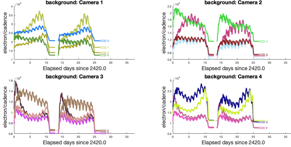
Figure 2: Median background flux across all targets on a given CCD in each camera. The changes are caused by variations in the orientation and distance of the Earth and Moon.
