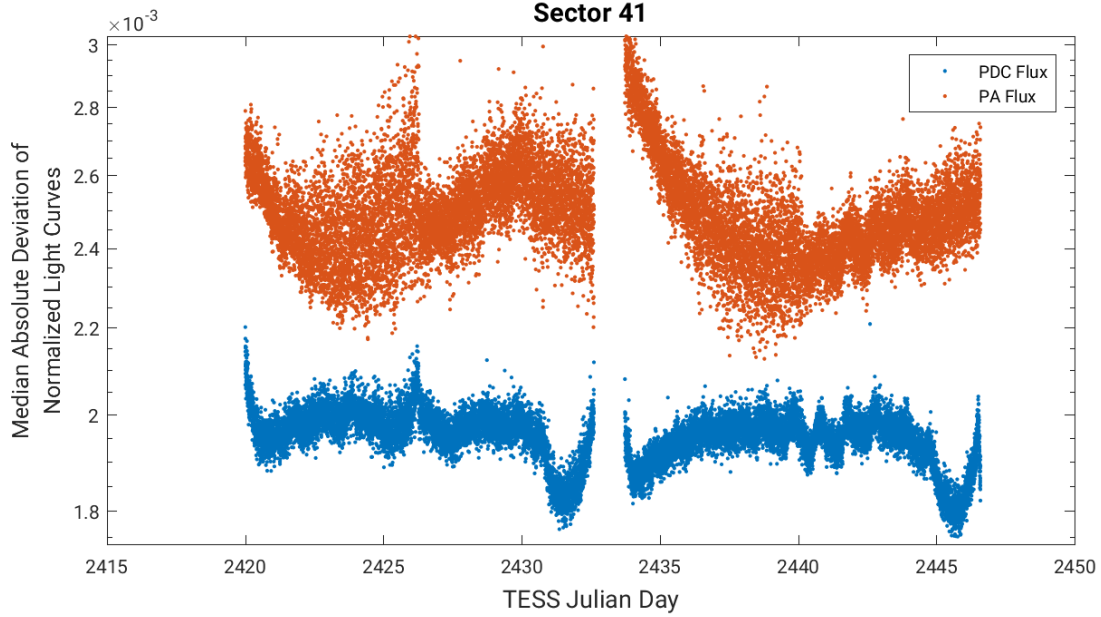
Figure 4: Median absolute deviation (MAD) for the two-minute cadence data from Sector 41, showing the performance of the cotrending after identifying Manual Exclude data quality flags. The MAD is calculated in each cadence across stars with flux variations less than 1% for both the PA (red) and PDC (blue) light curves, where each light curve is normalized by its median flux value. The scatter in the PA light curves is much higher than that for the PDC light curves, and the outliers in the PA light curves are largely absent from the PDC light curves due to the use of the anomaly flags.
