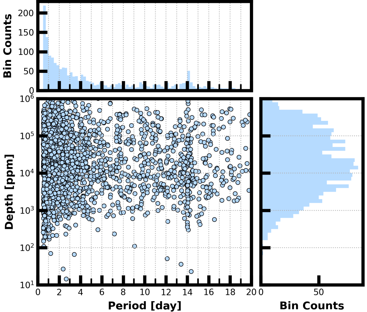
Figure 8: Lower Left Panel: Transit depth as a function of orbital period for the 2376 TCEs identified for the Sector 41 search. For enhanced visibility of long period detections, TCEs with orbital period < 0.5 days are not shown. Reported depth comes from the DV limb-darkened transit fit depth when available, and the DV trapezoid model fit depth when not available. Top Panel: Orbital period distribution of the TCEs shown in the lower left panel. Right Panel: Transit depth distribution for the TCEs shown in the lower left panel.
