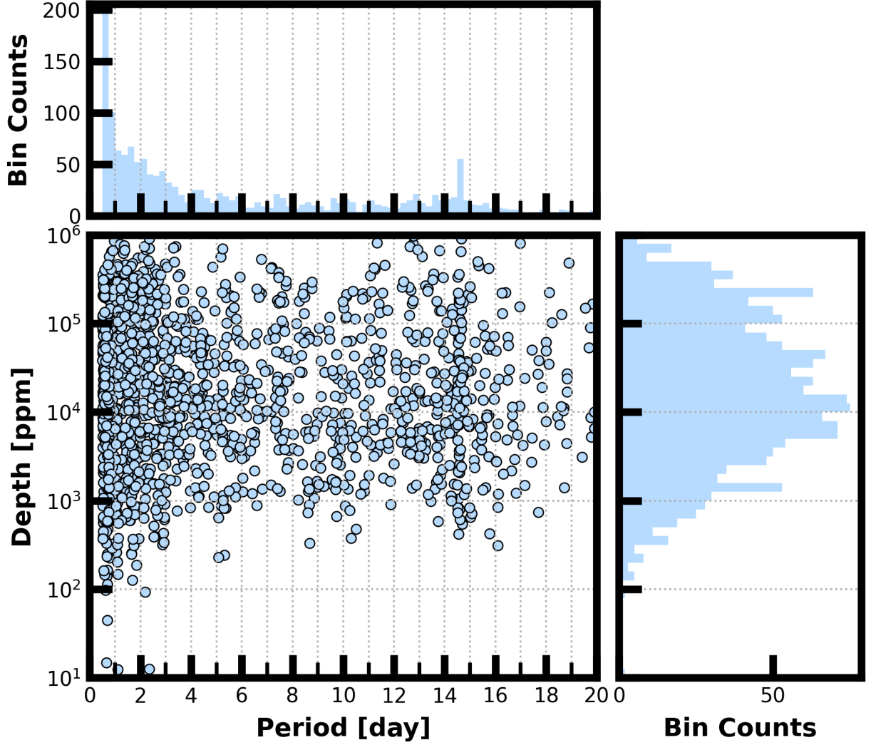
Figure 8: Lower Left Panel: Transit depth as a function of orbital period for the 2051 TCEs identified for the Sector 40 search. For enhanced visibility of long period detections, TCEs with orbital period < 0.5 days are not shown. Reported depth comes from the DV limb-darkened transit fit depth when available, and the DV trapezoid model fit depth when not available. Top Panel: Orbital period distribution of the TCEs shown in the lower left panel. Right Panel: Transit depth distribution for the TCEs shown in the lower left panel.
