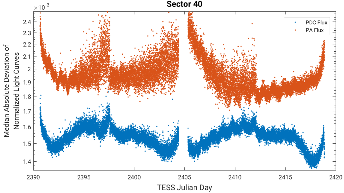
Figure 4: Median absolute deviation (MAD) for the two-minute cadence data from Sector 40, showing the performance of the cotrending after identifying Manual Exclude data quality flags. The MAD is calculated in each cadence across stars with flux variations less than 1% for both the PA (red) and PDC (blue) light curves, where each light curve is normalized by its median flux value. The scatter in the PA light curves is much higher than that for the PDC light curves, and the outliers in the PA light curves are largely absent from the PDC light curves due to the use of the anomaly flags.
