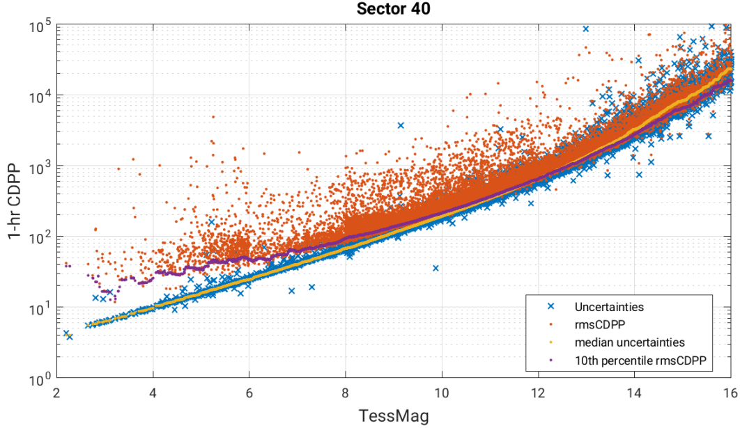
Figure 6: 1-hour CDPP. The red points are the RMS CDPP measurements for the 19995 light curves from Sector 40 plotted as a function of TESS magnitude. The blue x’s are the uncertainties, scaled to 1-hour timescale. The purple curve is a moving 10th percentile of the RMS CDPP measurements, and the gold curve is a moving median of the 1-hr uncertainties.
