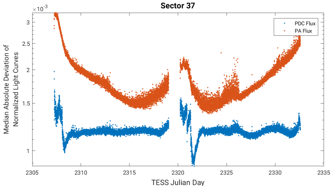
Figure 4: Median absolute deviation (MAD) for the two-minute cadence data from Sector 37, showing the performance of the cotrending after identifying Manual Exclude data quality flags. The MAD is calculated in each cadence across stars with flux variations less than 1% for both the PA (red) and PDC (blue) light curves, where each light curve is normalized by its median flux value. The scatter in the PA light curves is much higher than that for the PDC light curves, and the outliers in the PA light curves are largely absent from the PDC light curves due to the use of the anomaly flags.
