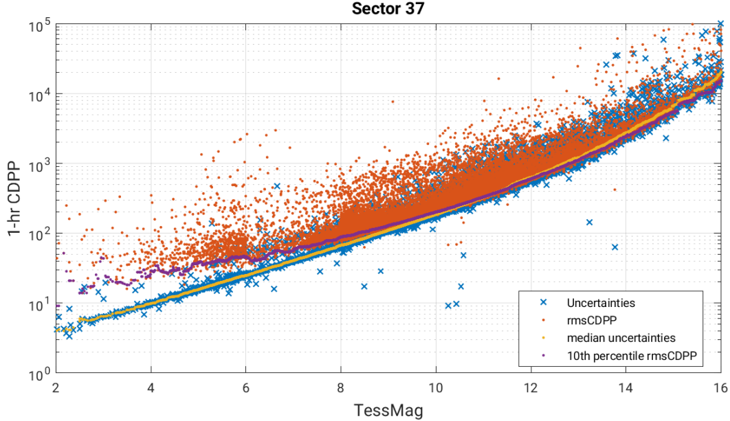
Figure 6: 1-hour CDPP. The red points are the RMS CDPP measurements for the 19991 light curves from Sector 37 plotted as a function of TESS magnitude. The blue x’s are the uncertainties, scaled to 1-hour timescale. The purple curve is a moving 10th percentile of the RMS CDPP measurements, and the gold curve is a moving median of the 1-hr uncertainties.
