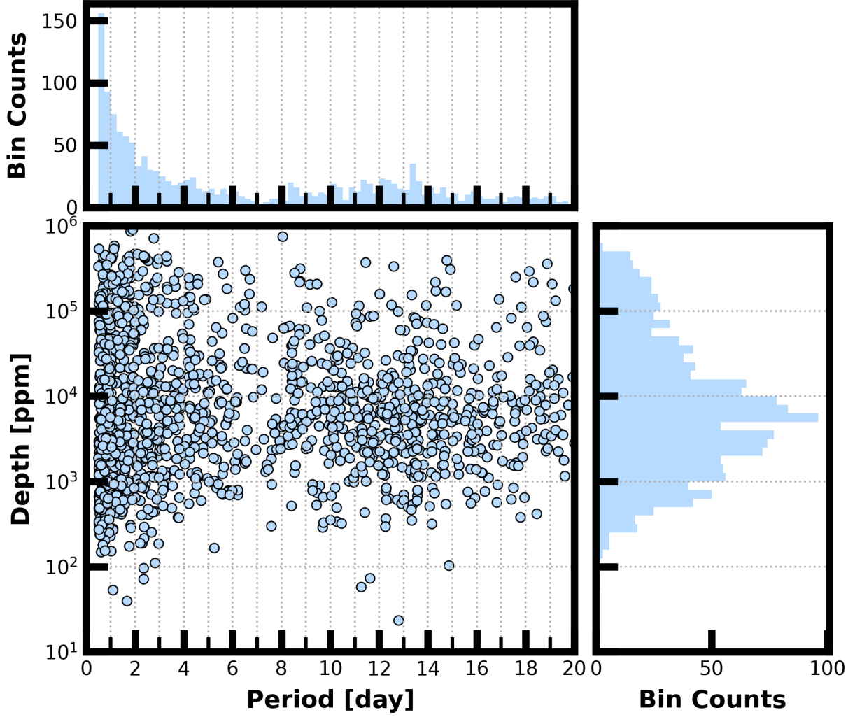
Figure 8: Lower Left Panel: Transit depth as a function of orbital period for the 1879 TCEs identified for the Sector 37 search. For enhanced visibility of long period detections, TCEs with orbital period < 0.5 days are not shown. Reported depth comes from the DV limb-darkened transit fit depth when available, and the DV trapezoid model fit depth when not available. Top Panel: Orbital period distribution of the TCEs shown in the lower left panel. Right Panel: Transit depth distribution for the TCEs shown in the lower left panel.
