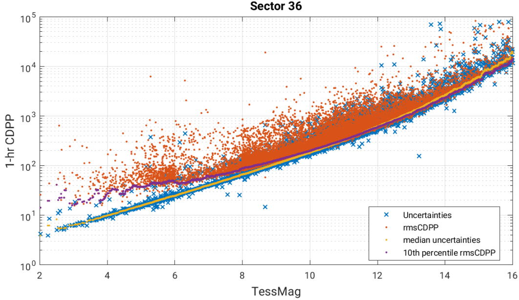
Figure 6: 1-hour CDPP. The red points are the RMS CDPP measurements for the 19993 light curves from Sector 36 plotted as a function of TESS magnitude. The blue x’s are the uncertainties, scaled to 1-hour timescale. The purple curve is a moving 10th percentile of the RMS CDPP measurements, and the gold curve is a moving median of the 1-hr uncertainties.
