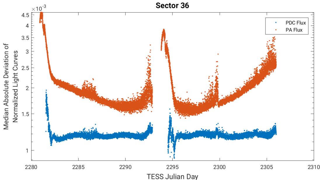
Figure 4: Median absolute deviation (MAD) for the two-minute cadence data from Sector 36, showing the performance of the cotrending after identifying Manual Exclude data quality flags. The MAD is calculated in each cadence across stars with flux variations less than 1% for both the PA (red) and PDC (blue) light curves, where each light curve is normalized by its median flux value. The scatter in the PA light curves is much higher than that for the PDC light curves, and the outliers in the PA light curves are largely absent from the PDC light curves due to the use of the anomaly flags.
