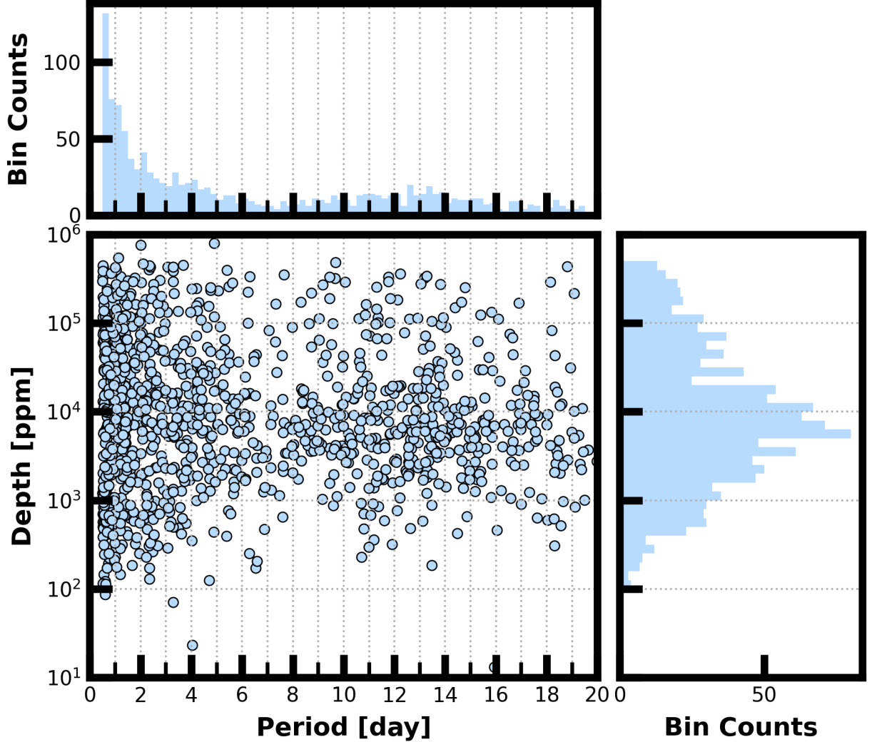
Figure 8: Lower Left Panel: Transit depth as a function of orbital period for the 1544 TCEs identified for the Sector 36 search. For enhanced visibility of long period detections, TCEs with orbital period < 0.5 days are not shown. Reported depth comes from the DV limb-darkened transit fit depth when available, and the DV trapezoid model fit depth when not available. Top Panel: Orbital period distribution of the TCEs shown in the lower left panel. Right Panel: Transit depth distribution for the TCEs shown in the lower left panel.
