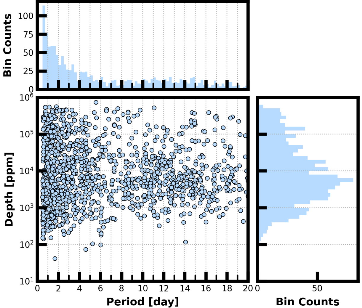
Figure 8: Lower Left Panel: Transit depth as a function of orbital period for the 1670 TCEs identified for the Sector 34 search. For enhanced visibility of long period detections, TCEs with orbital period < 0.5 days are not shown. Reported depth comes from the DV limb-darkened transit fit depth when available, and the DV trapezoid model fit depth when not available. Top Panel: Orbital period distribution of the TCEs shown in the lower left panel. Right Panel: Transit depth distribution for the TCEs shown in the lower left panel.
