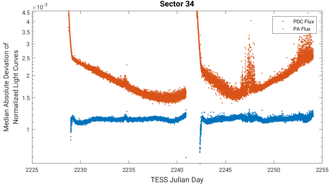
Figure 4: Median absolute deviation (MAD) for the two-minute cadence data from Sector 34, showing the performance of the cotrending after identifying Manual Exclude data quality flags. The MAD is calculated in each cadence across stars with flux variations less than 1% for both the PA (red) and PDC (blue) light curves, where each light curve is normalized by its median flux value. The scatter in the PA light curves is much higher than that for the PDC light curves, and the outliers in the PA light curves are largely absent from the PDC light curves due to the use of the anomaly flags.
