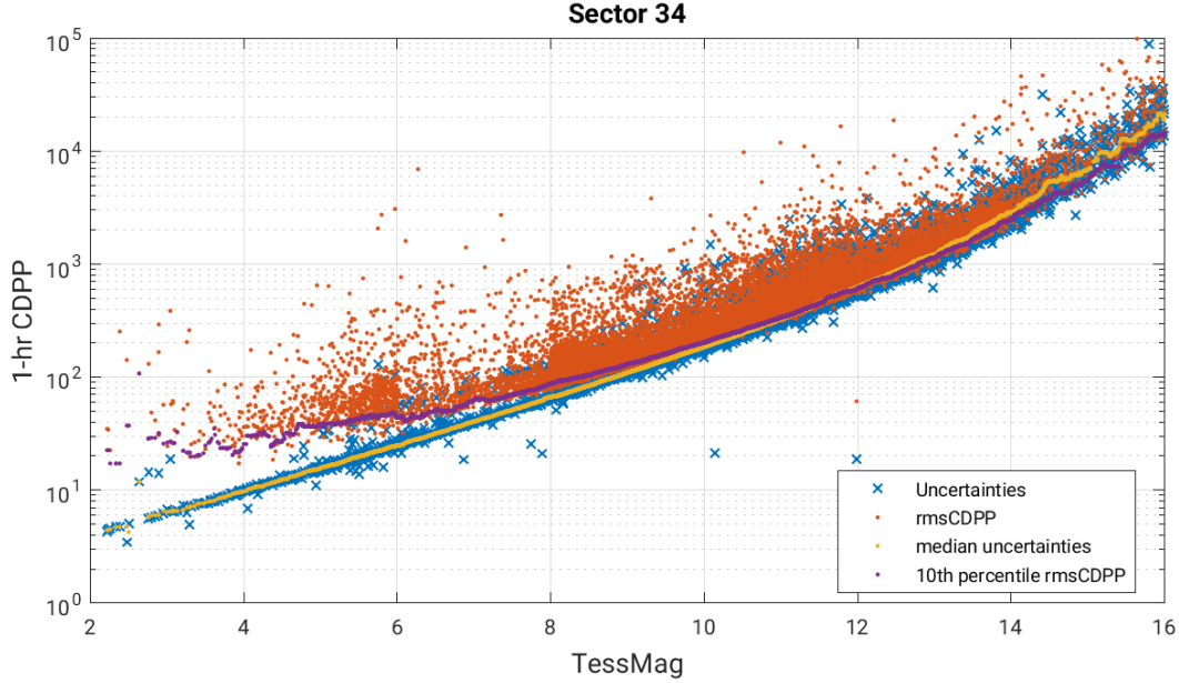
Figure 6: 1-hour CDPP. The red points are the RMS CDPP measurements for the 19993 light curves from Sector 34 plotted as a function of TESS magnitude. The blue x’s are the uncertainties, scaled to 1-hour timescale. The purple curve is a moving 10th percentile of the RMS CDPP measurements, and the gold curve is a moving median of the 1-hr uncertainties.
