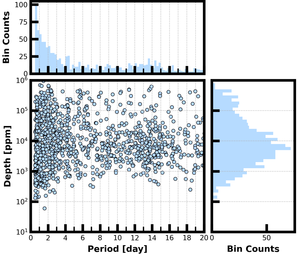
Figure 8: Lower Left Panel: Transit depth as a function of orbital period for the 1522 TCEs identified for the Sector 33 search. For enhanced visibility of long period detections, TCEs with orbital period < 0.5 days are not shown. Reported depth comes from the DV limb-darkened transit fit depth when available, and the DV trapezoid model fit depth when not available. Top Panel: Orbital period distribution of the TCEs shown in the lower left panel. Right Panel: Transit depth distribution for the TCEs shown in the lower left panel.
