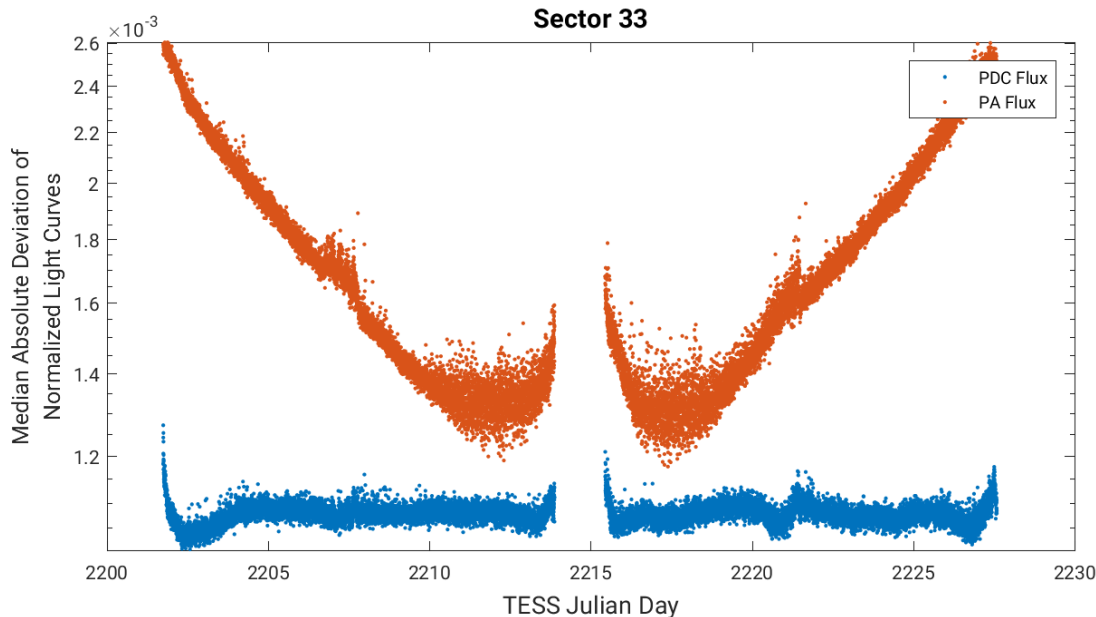
Figure 4: Median absolute deviation (MAD) for the two-minute cadence data from Sector 33, showing the performance of the cotrending after identifying Manual Exclude data quality flags. The MAD is calculated in each cadence across stars with flux variations less than 1% for both the PA (red) and PDC (blue) light curves, where each light curve is normalized by its median flux value. The scatter in the PA light curves is much higher than that for the PDC light curves, and the outliers in the PA light curves are largely absent from the PDC light curves due to the use of the anomaly flags.
