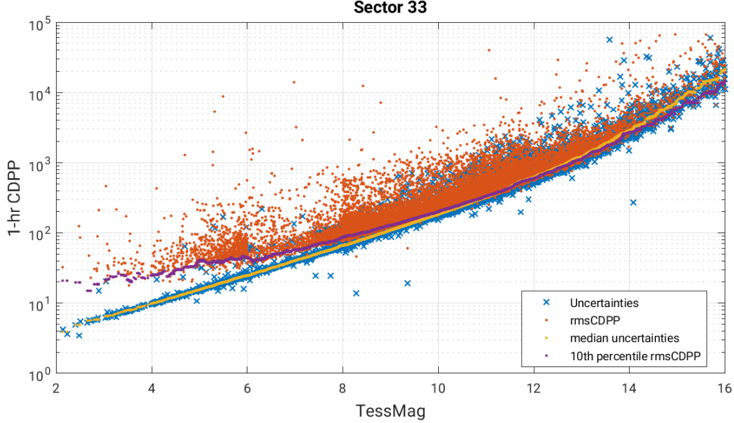
Figure 6: 1-hour CDPP. The red points are the RMS CDPP measurements for the 19991 light curves from Sector 33 plotted as a function of TESS magnitude. The blue x’s are the uncertainties, scaled to 1-hour timescale. The purple curve is a moving 10th percentile of the RMS CDPP measurements, and the gold curve is a moving median of the 1-hr uncertainties.
