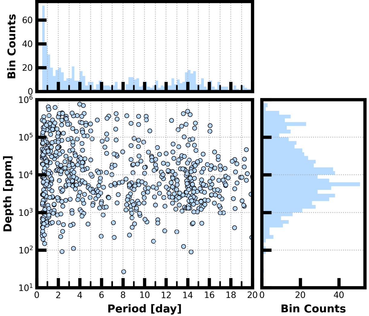
Figure 8: Lower Left Panel: Transit depth as a function of orbital period for the 921 TCEs identified for the Sector 30 search. For enhanced visibility of long period detections, TCEs with orbital period < 0.5 days are not shown. Reported depth comes from the DV limb-darkened transit fit depth when available, and the DV trapezoid model fit depth when not available. Top Panel: Orbital period distribution of the TCEs shown in the lower left panel. Right Panel: Transit depth distribution for the TCEs shown in the lower left panel.
