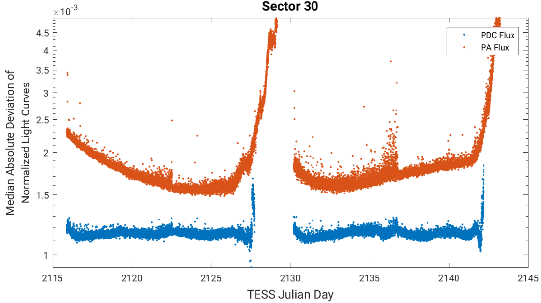
Figure 4: Median absolute deviation (MAD) for the two-minute cadence data from Sector 30, showing the performance of the cotrending after identifying Manual Exclude data quality flags. The MAD is calculated in each cadence across stars with flux variations less than 1% for both the PA (red) and PDC (blue) light curves, where each light curve is normalized by its median flux value. The scatter in the PA light curves is much higher than that for the PDC light curves, and the outliers in the PA light curves are largely absent from the PDC light curves due to the use of the anomaly flags.
