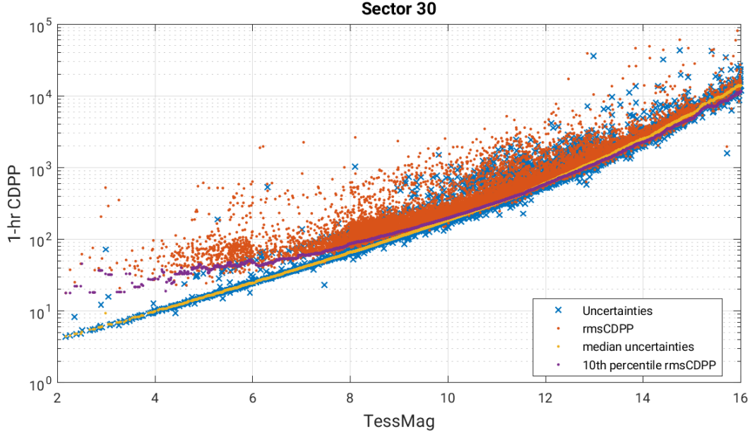
Figure 6: 1-hour CDPP. The red points are the RMS CDPP measurements for the 19,996 light curves from Sector 30 plotted as a function of TESS magnitude. The blue x’s are the uncertainties, scaled to 1-hour timescale. The purple curve is a moving 10th percentile of the RMS CDPP measurements, and the gold curve is a moving median of the 1-hr uncertainties.
