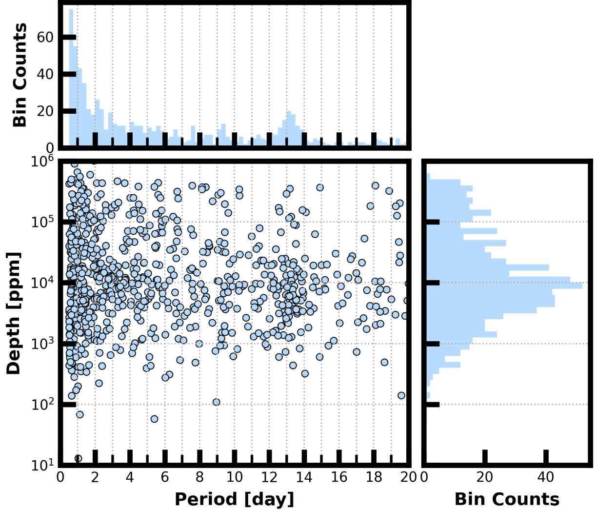
Figure 8: Lower Left Panel: Transit depth as a function of orbital period for the 909 TCEs identified for the Sector 28 search. For enhanced visibility of long period detections, TCEs with orbital period < 0.5 days are not shown. Reported depth comes from the DV limb-darkened transit fit depth when available, and the DV trapezoid model fit depth when not available. Top Panel: Orbital period distribution of the TCEs shown in the lower left panel. Right Panel: Transit depth distribution for the TCEs shown in the lower left panel.
