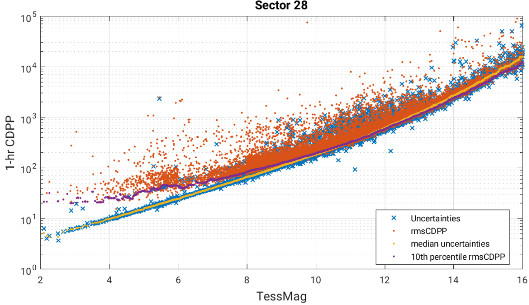
Figure 6: 1-hour CDPP. The red points are the RMS CDPP measurements for the 19,994 light curves from Sector 28 plotted as a function of TESS magnitude. The blue x’s are the uncertainties, scaled to 1-hour timescale. The purple curve is a moving 10th percentile of the RMS CDPP measurements, and the gold curve is a moving median of the 1-hr uncertainties.
