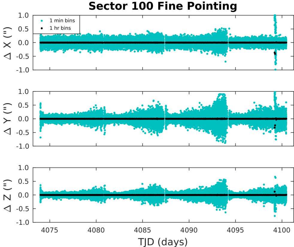
Figure 1: The delta-quaternions from each camera have been converted to spacecraft frame, binned to 1 minute and 1 hour, averaged across cameras. Long-term trends (such as those caused by differential velocity aberration) have also been removed. The \Delta X/\Delta Y directions represent offsets along the detectors’ rows/columns, while the \Delta Z direction represents spacecraft roll.
