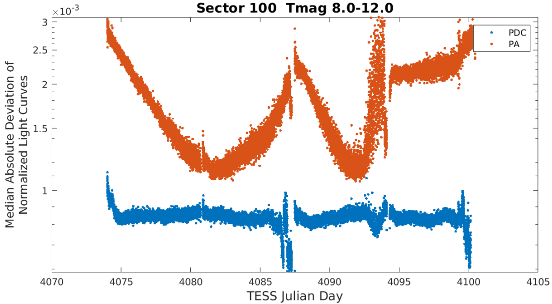
Figure 4: Median absolute deviation (MAD) for the two-minute cadence data from Sector 100, showing the performance of the cotrending after identifying Manual Exclude data quality flags. The MAD is calculated in each cadence across stars with flux variations less than 1% for both the PA (red) and PDC (blue) light curves, where each light curve is normalized by its median flux value. The scatter in the PA light curves is much higher than that for the PDC light curves, and the outliers in the PA light curves are largely absent from the PDC light curves due to the use of the anomaly flags.
