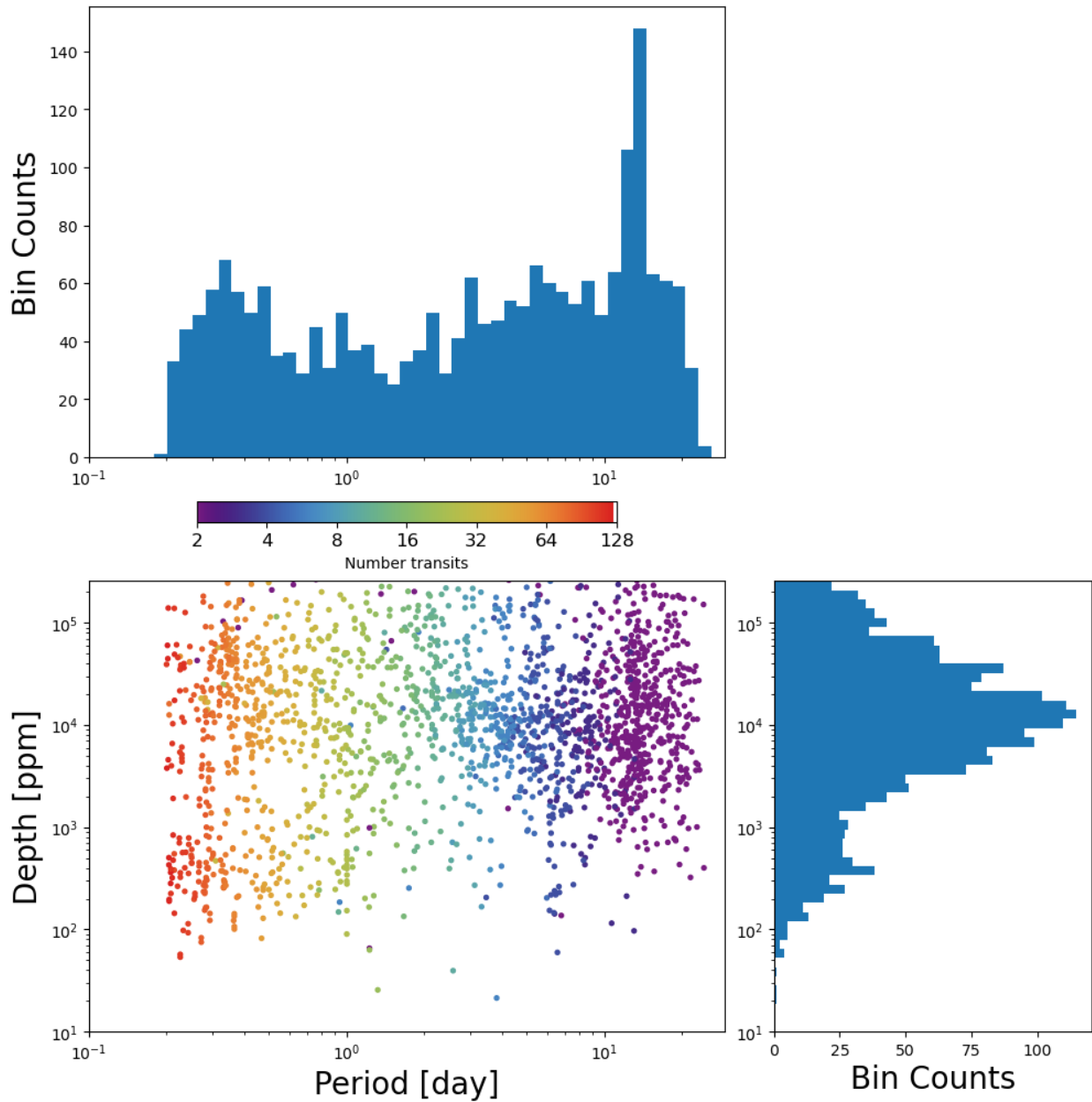
Figure 7: Lower Left Panel: Transit depth as a function of orbital period for the 2108 TCEs identified for the Sector 100 search. Reported depth comes from the DV limb-darkened transit fit depth when available, and the DV trapezoid model fit depth when not available. The number of observed transit events for each TCE is indicated by point color. Top Panel: Orbital period distribution of the TCEs shown in the lower left panel. Right Panel: Transit depth distribution for the TCEs shown in the lower left panel.
