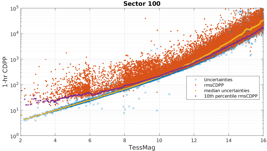
Figure 5: 1-hour CDPP. The red points are the RMS CDPP measurements for the 12988 light curves from Sector 100 plotted as a function of TESS magnitude. The blue x’s are the uncertainties, scaled to 1-hour timescale. The purple curve is a moving 10th percentile of the RMS CDPP measurements, and the gold curve is a moving median of the 1-hr uncertainties.
