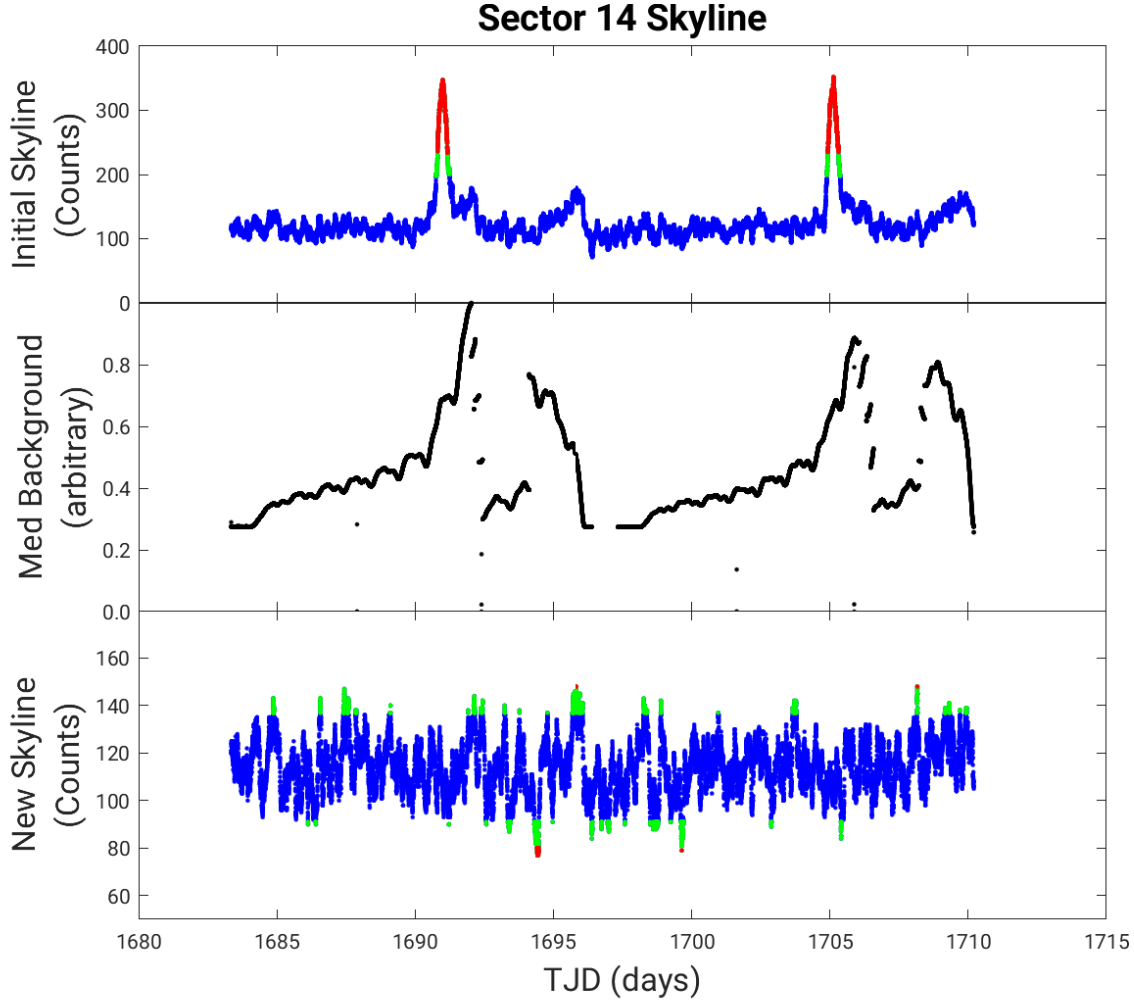
Figure 1: Comparison of TPS results before and after reprocessing, using Sector 14 as an example. Top panel: Number of TCEs in transit for each cadence in Sector 14, the so-called "skyline figure," from the initial data release. These data are from the first iteration of TPS, before any deemphasis weights are applied (see §4.2 of DRN19). The blue, green, and red points show the 1, 2, and 3\sigma outliers, respectively. The large spikes indicate times when many TCEs show a transit signal, marking cadences affected by systematic errors. Middle panel: Median background flux across all targets as a function of time. The increase in the background level towards the end of each orbit is caused by the proximity of the Earth to the camera fields-of-view. In the initial data release, scattered light flags were set for all targets on a given CCD during the times with the largest background levels. These flags cause a deep drop in the median background from approximately TJD 1692 to 1694 and from TJD 1707 to 1709. The excess of TCEs in the top panel is correlated with the initial increase in the background level, and then falls off when the scattered light flags are applied. Bottom panel: Same as top panel but for DR30, using target-by-target automated scattered light flags (see §2.4). No correlation with the median background exists, showing how the improved scattered light flags suppress the systematic errors in the transit search.
